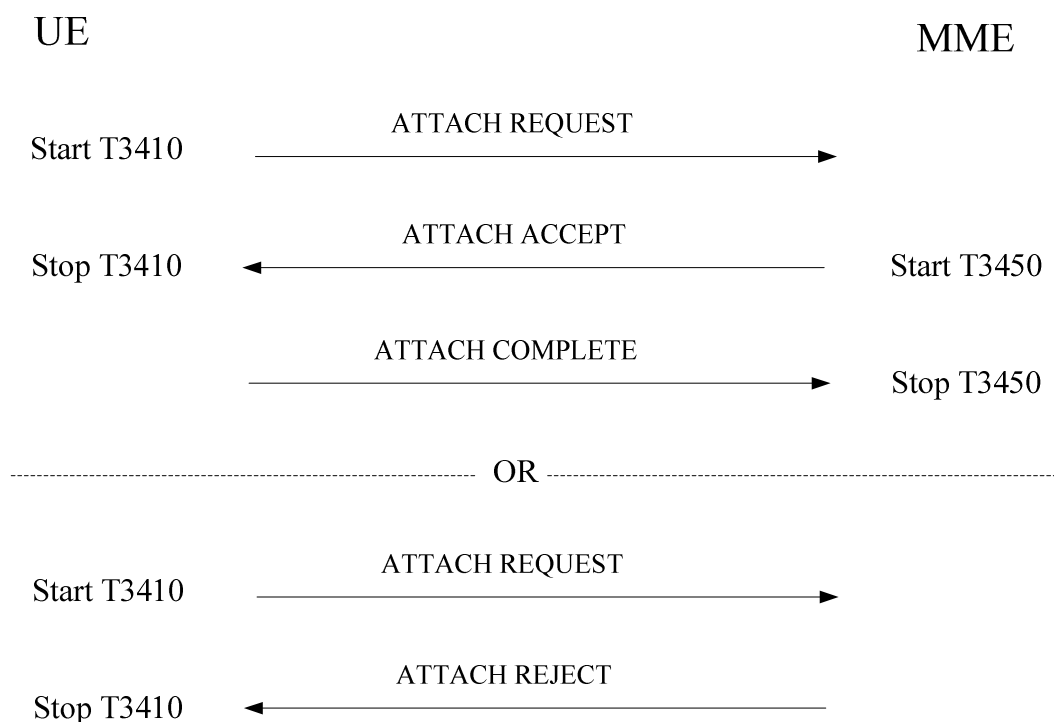
Figure 5.5.1.2.2.1: Attach procedure and combined attach procedure
