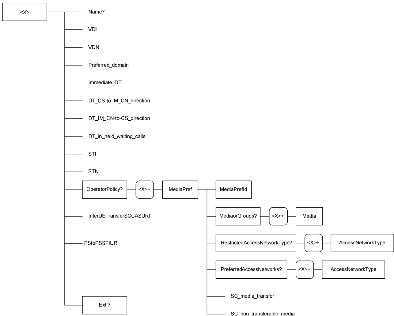
Figure 1: The Communication Continuity Object
