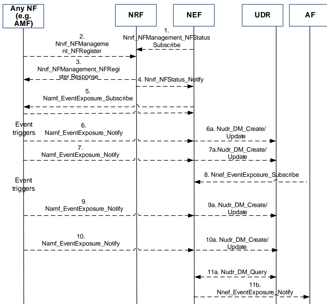
Figure 4.15.3.2.4-1: NF registration/status notification and Exposure with bulk subscription
