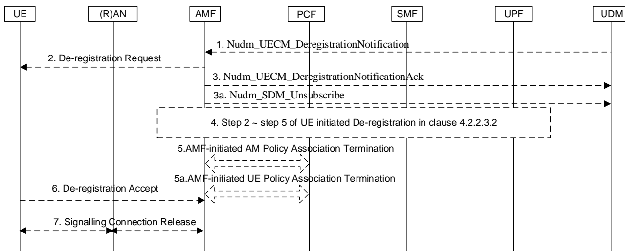
Figure 4.2.2.3.3-1: Network-initiated Deregistration
