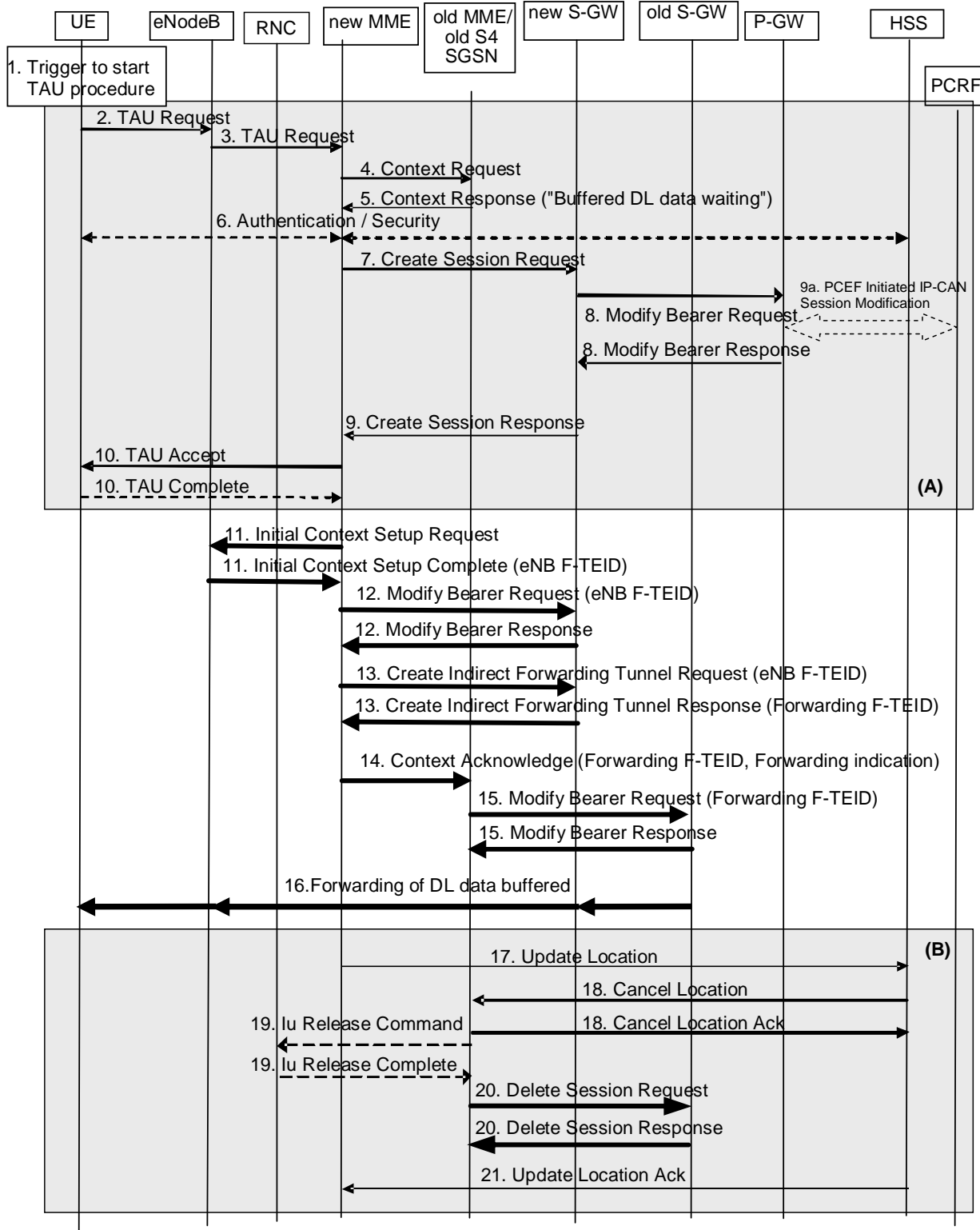
Figure 5.3.3.1A-1: Tracking Area Update procedure with Serving GW change and data forwarding
