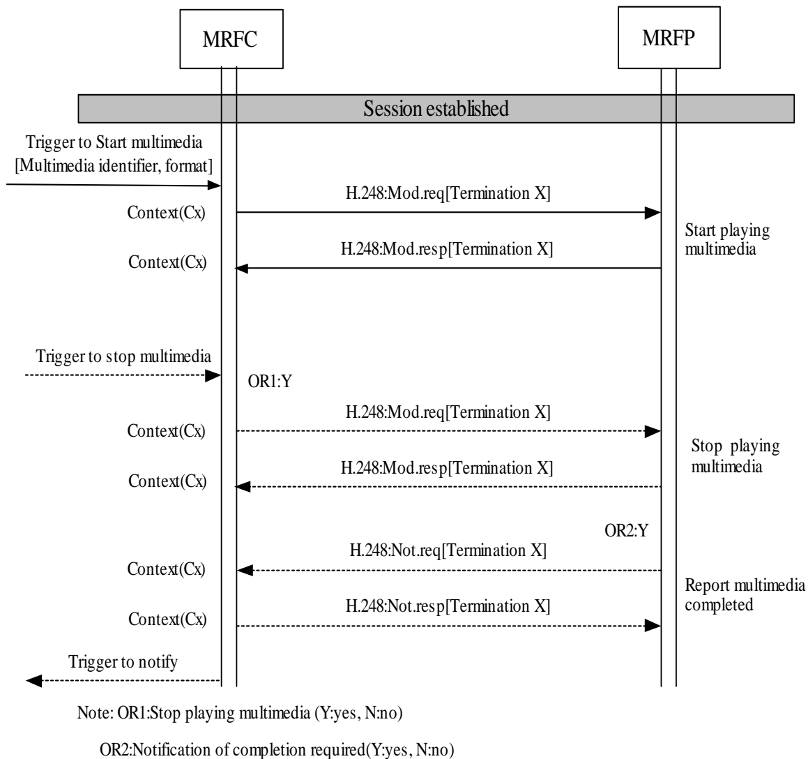
Figure 6.2.7.2 Play multimedia (message sequence chart)
