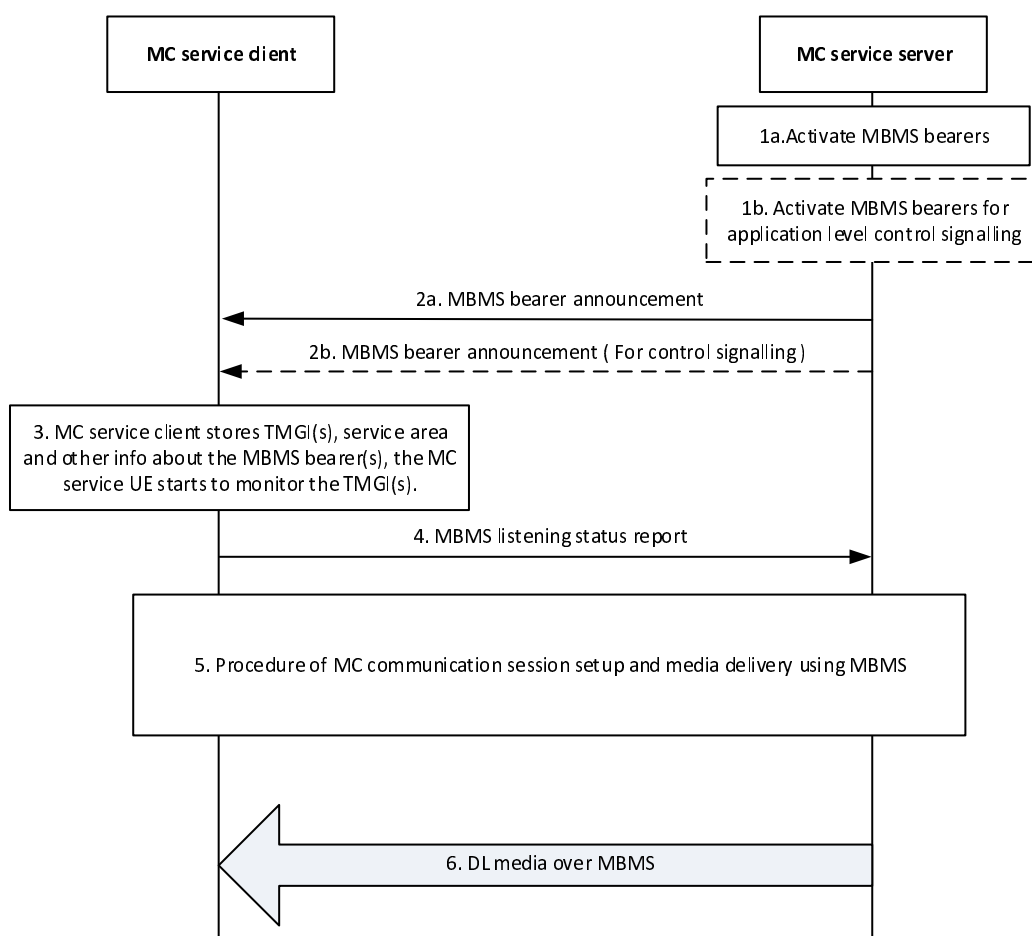
Figure 10.7.3.1.2-1: Use of pre-established MBMS bearers
