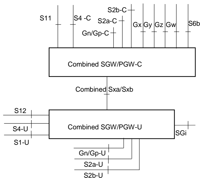
Figure 4.2.2-1: Architecture reference model with separation of user plane and control plane for a combined SGW/PGW
