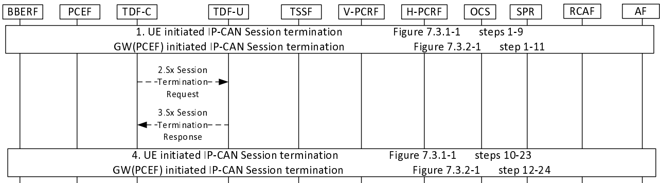
Figure 6.3.2.2-1: Interaction between CP and UP function with IP-CAN session termination
