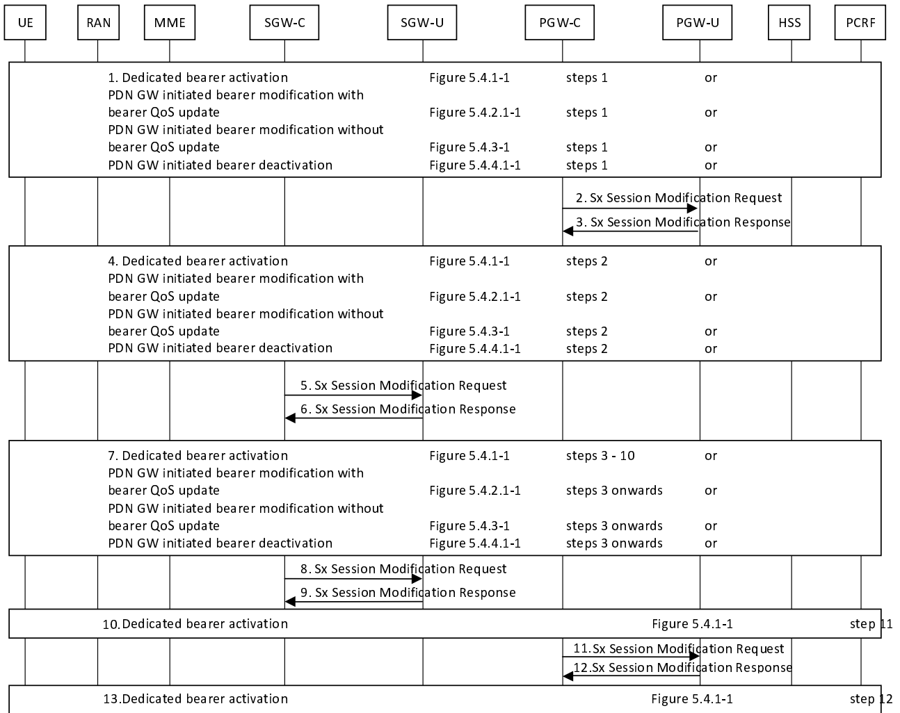
Figure 6.3.1.7-1: Interaction between CP and UP function during modification of bearer
