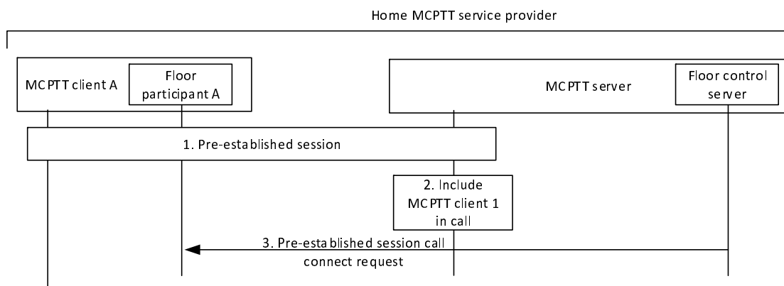
Figure 10.5.3.5.1-1: Connect procedure
