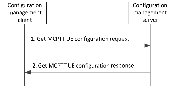
Figure 10.1.3.2-1: MCPTT UE obtains the configuration data
