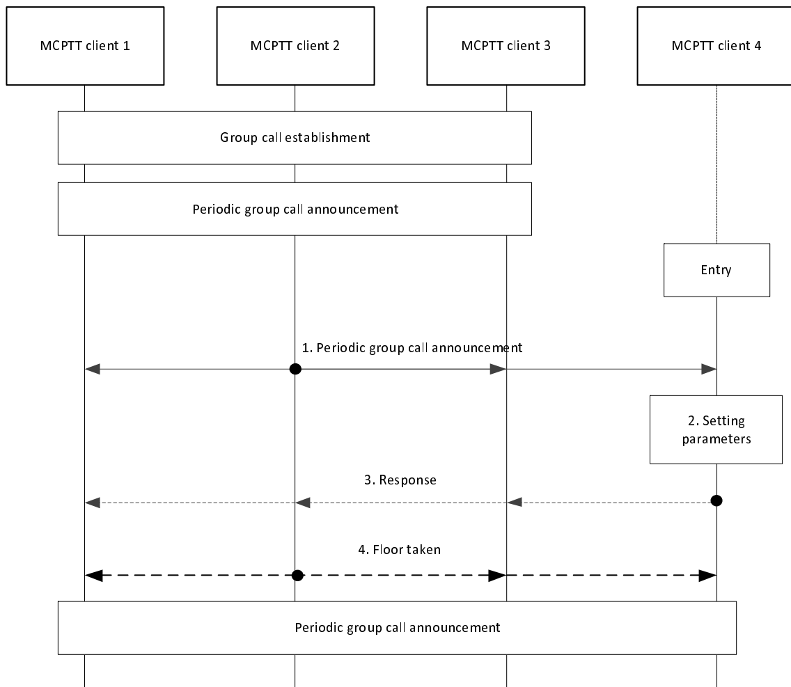
Figure 10.6.3.4-1: Passive join to group call
