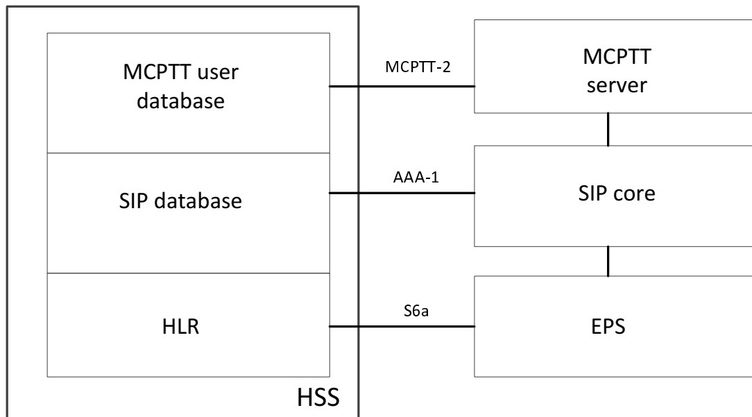
Figure 9.2.2.2-1: Collocation of MCPTT user database and SIP database with HSS
