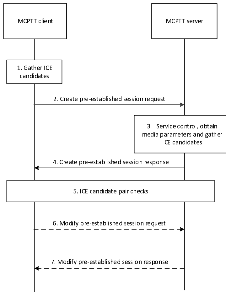
Figure 10.5.3.2-1: Pre-established session establishment
