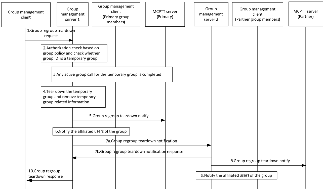
Figure 10.4.4.3-1: Temporary group tear down
