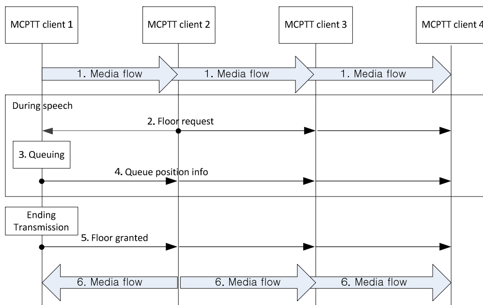
Figure 10.9.2.5-1: Floor request during speaking with queue
