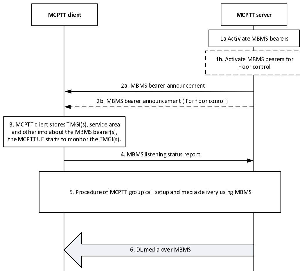
Figure 10.10.2.2-1: Use of pre-established MBMS bearers
