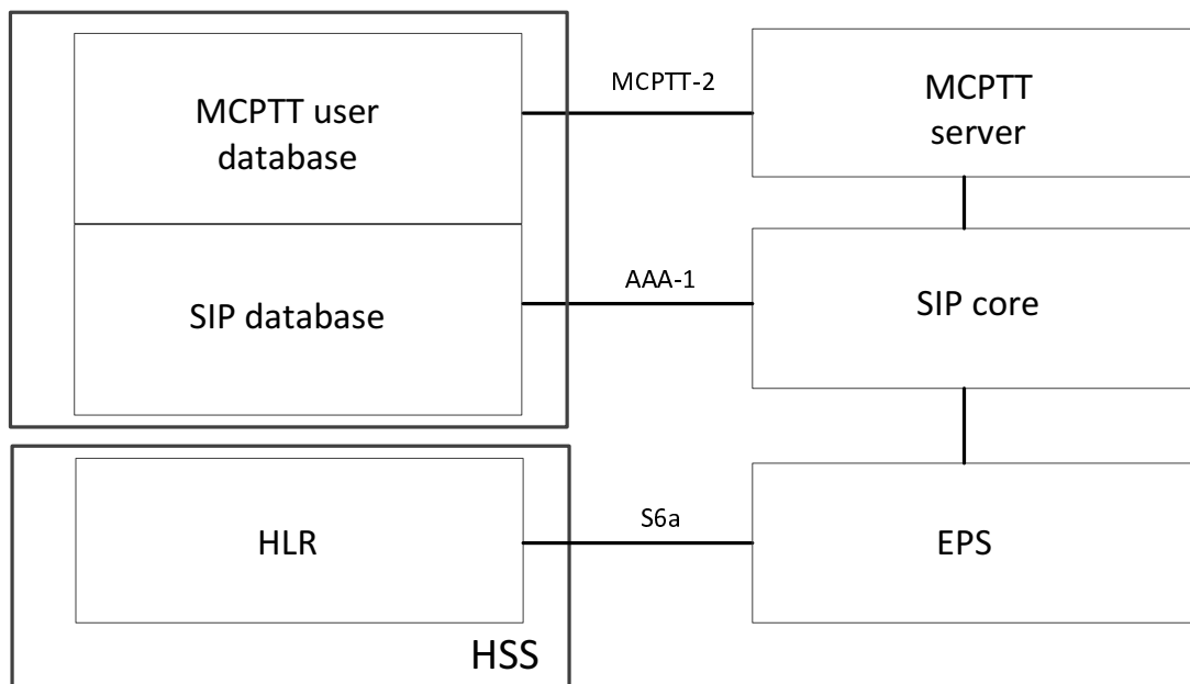
Figure 9.2.2.2-3: Shared PLMN operator and MCPTT service provider based deployment of MCPTT service - MCPTT user database and SIP database deployed together, with separate HSS
