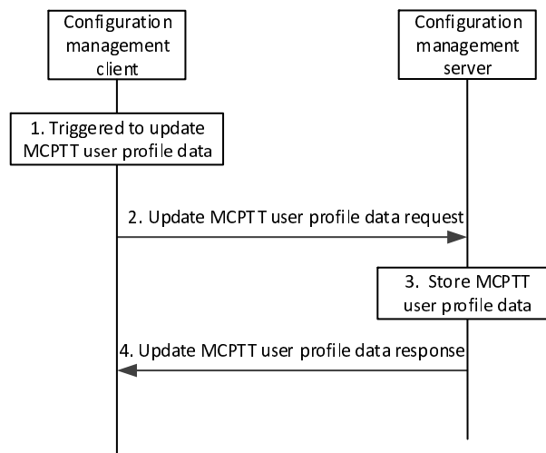
Figure 10.1.4.4-1: MCPTT user updates the MCPTT user profile data to the network
