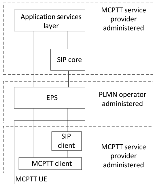
Figure 9.2.2.1.4-1: MCPTT service provider provision of SIP core, separate domain from EPS
