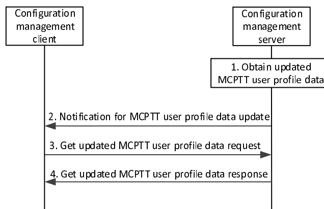
Figure 10.1.4.3-1: MCPTT user receives updated MCPTT user profile data from the network
