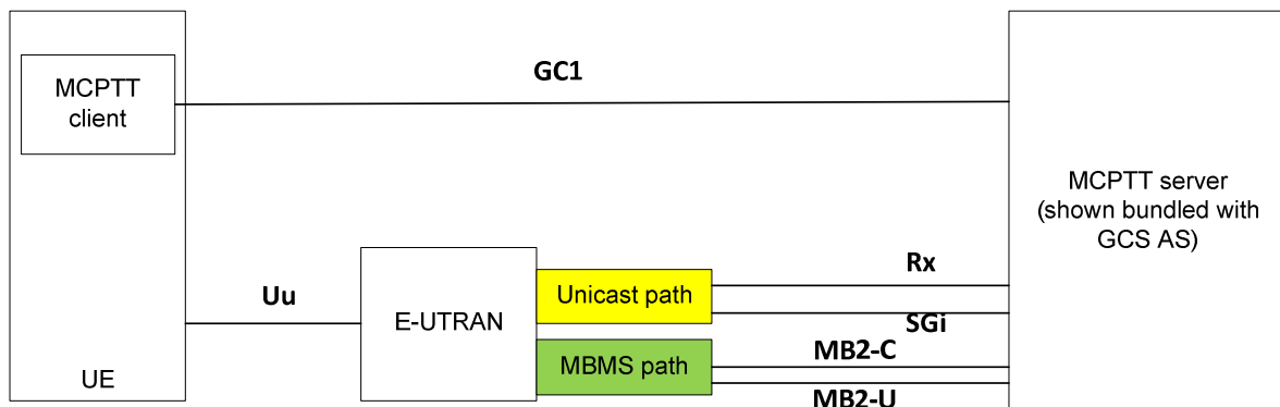
Figure 5.2.7-1: MCPTT on-network architecture showing MBMS
