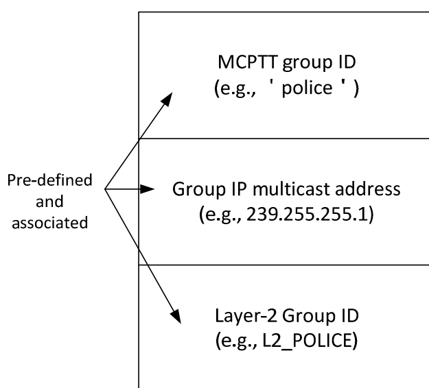
Figure 8.1.3.2-1: MCPTT group ID management in off-network operation
