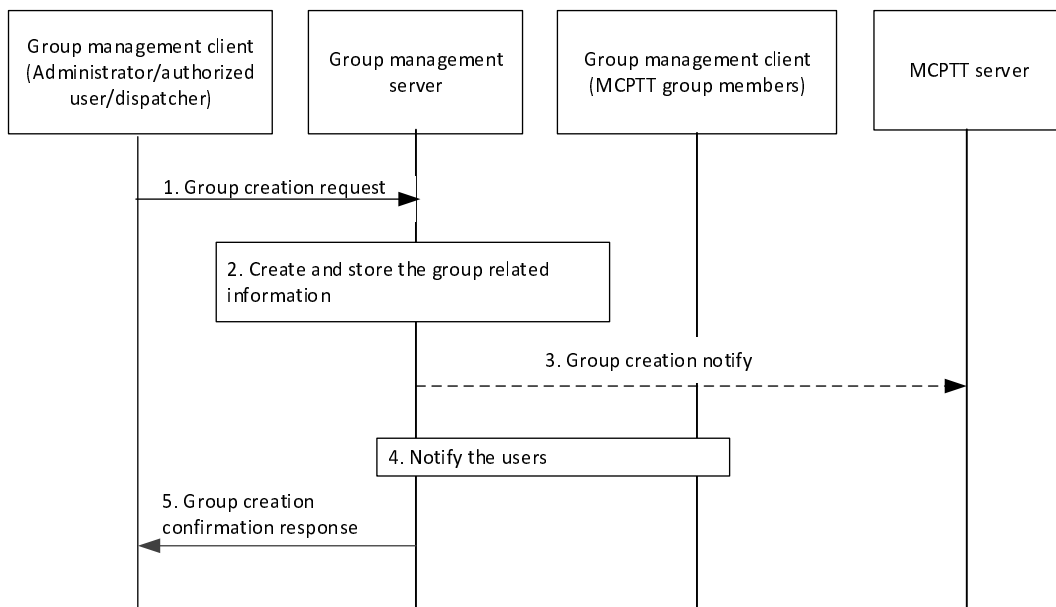
Figure 10.4.3-1: Group creation
