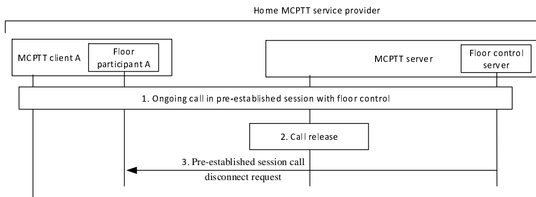
Figure 10.5.3.5.1-2: Disconnect procedure
