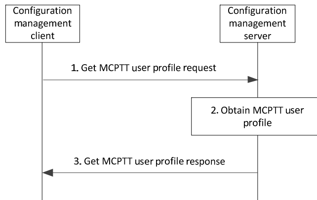
Figure 10.1.4.2-1: MCPTT user obtains the MCPTT user profile(s) from the network
