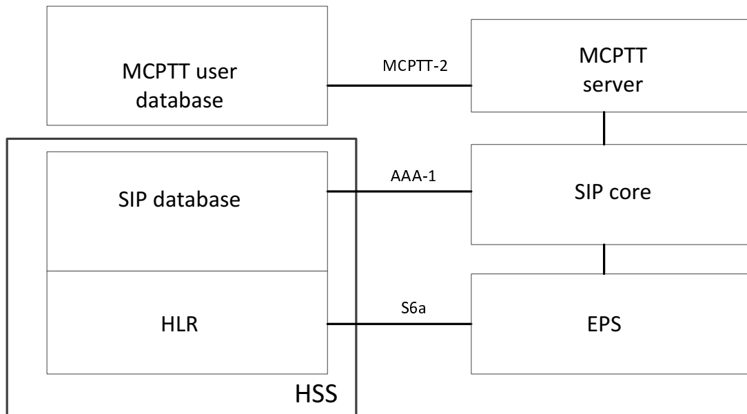
Figure 9.2.2.2-2: Shared PLMN operator and MCPTT service provider based deployment of MCPTT service - SIP database collocated with HSS with separate MCPTT user database
