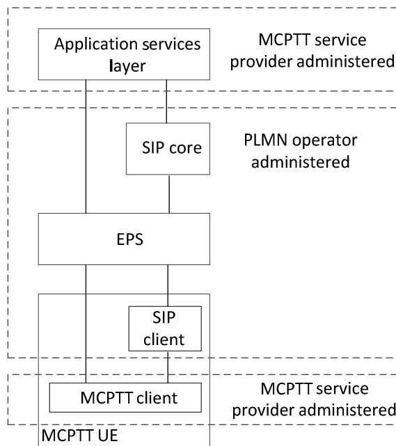
Figure 9.2.2.1.3-1: MCPTT service provider administers MCPTT service separately from SIP core and EPS
