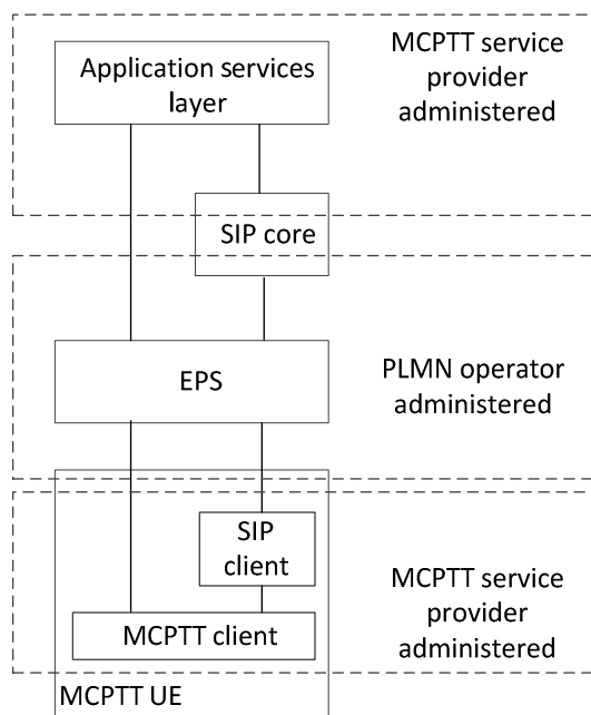
Figure 9.2.2.1.5-1: MCPTT service provider partial provision of SIP core, separate domain from EPS
