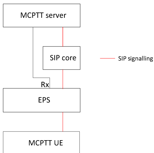
Figure 9.2.2.3.3-1: Bearer control by MCPTT server
