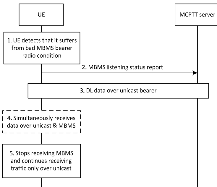
Figure 10.10.5-1: Switching from MBMS delivery to unicast delivery
