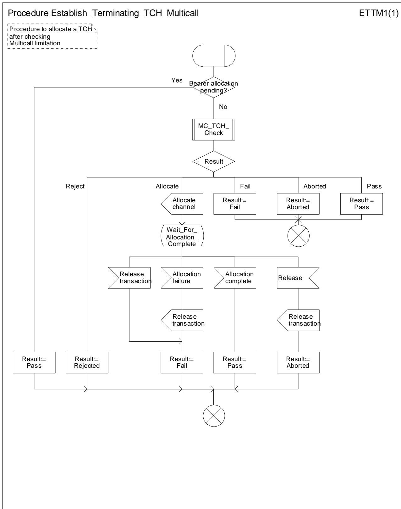
Figure 11: Procedure Establish_Terminating_TCH_Multicall
