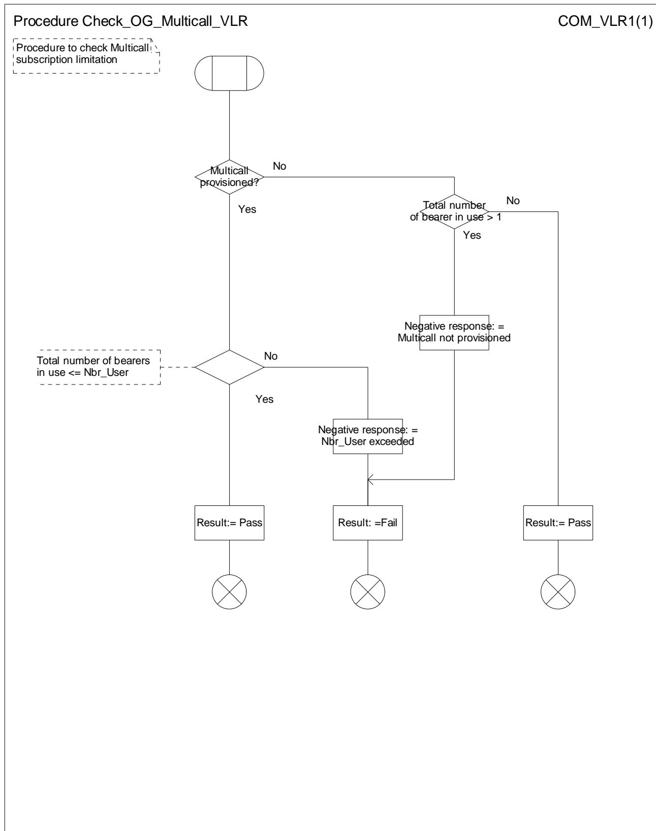
Figure 9: Procedure Check_OG_Multicall_VLR
