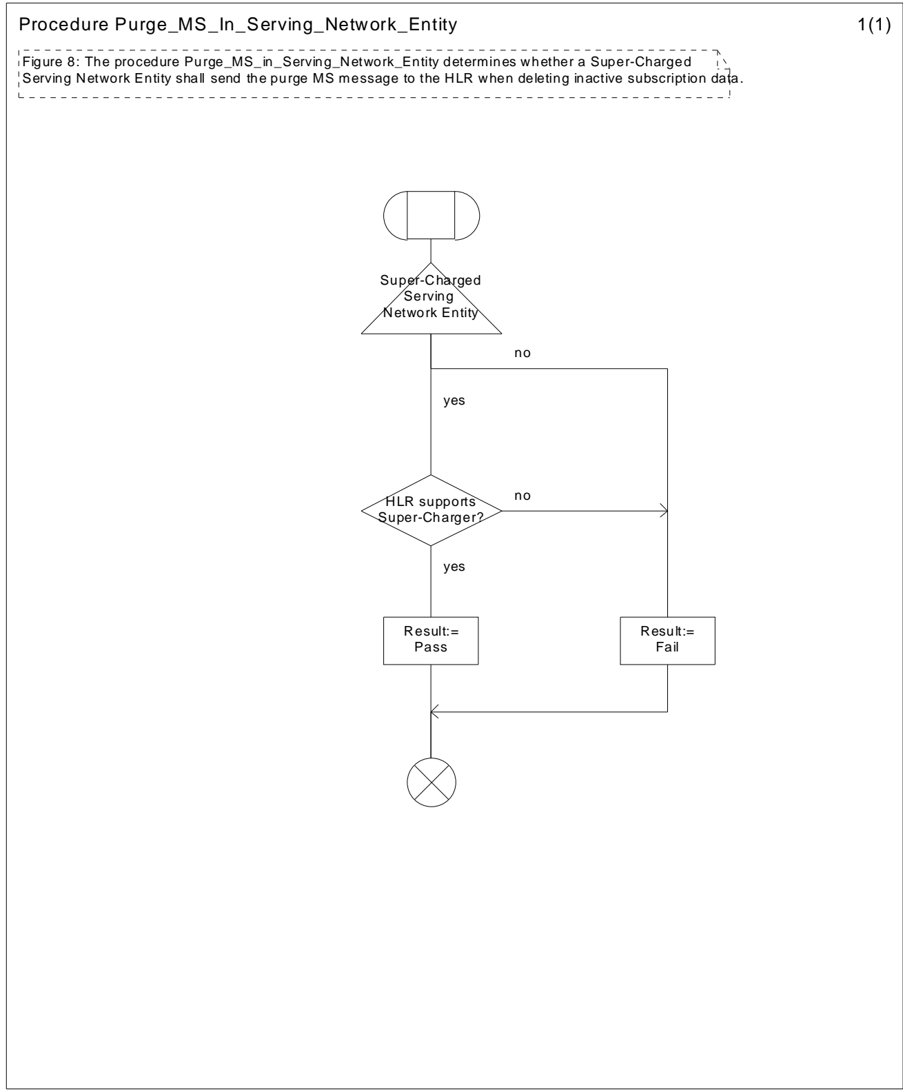
Figure 8: Procedure Purge_MS_In_Serving_Network_Entity
