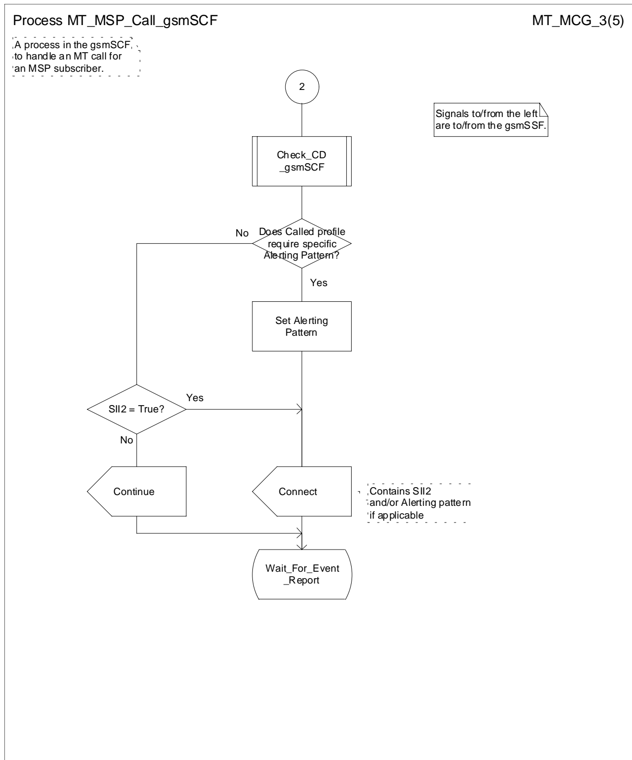
Figure 8c Error! Reference source not found.: Process MT_MSP_Call_gsmSCF (sheet 3 of 5)
