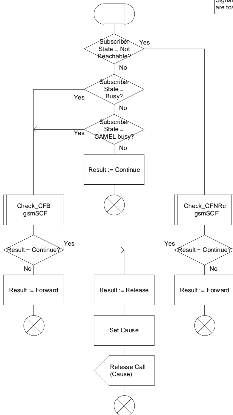
Figure 12: Procedure Check_Early_CF_gsmSCF
