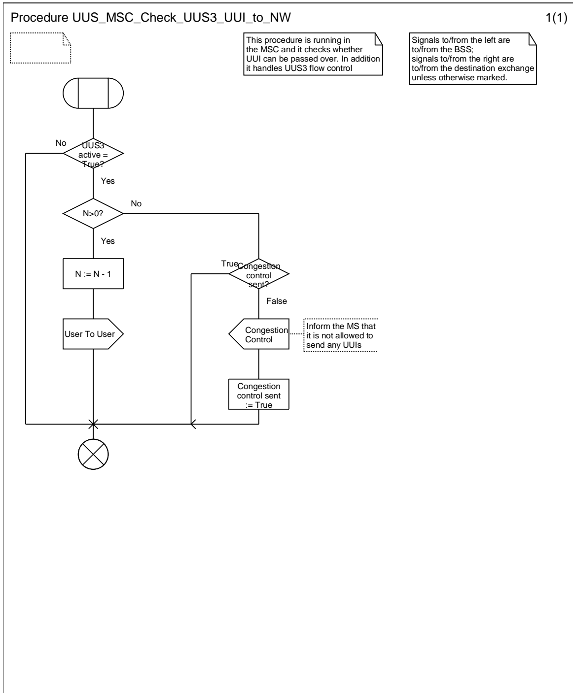
Figure 9.3.5: Procedure UUS_MSC_Check_UUS3_UUI_to_NW
