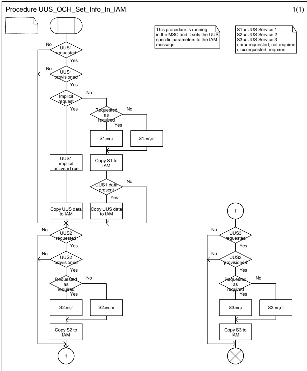
Figure 9.1.1.2: Procedure UUS_OCH_Set_Info_In_IAM
