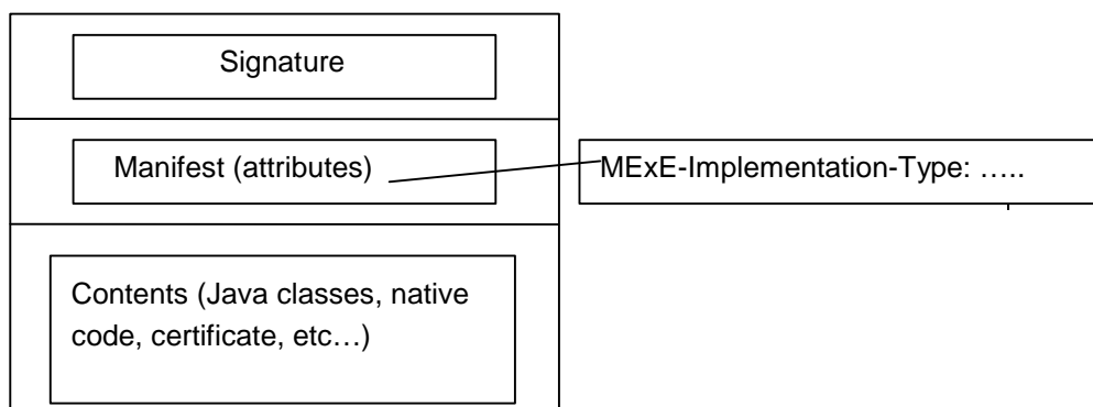
Figure 14: Signed packages
