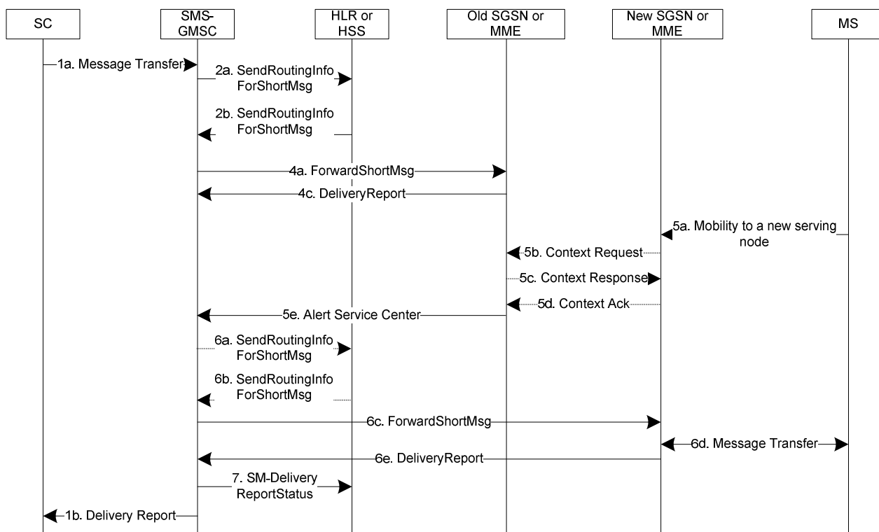
Figure 17c): Successful short message transfer attempt via the SGSN or MME, with short message retransmission by the SMS-GMSC upon MS mobility to a new serving node prior to the retransmission time requested by the SGSN or MME.
