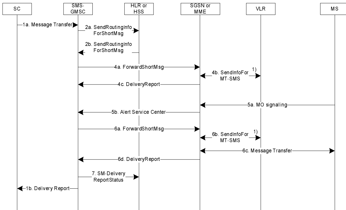
Figure 17b: Successful short message transfer attempt via the SGSN or MME, with short message retransmission by the SMS-GMSC upon MS originated signalling prior to the retransmission time requested by the SGSN or MME
