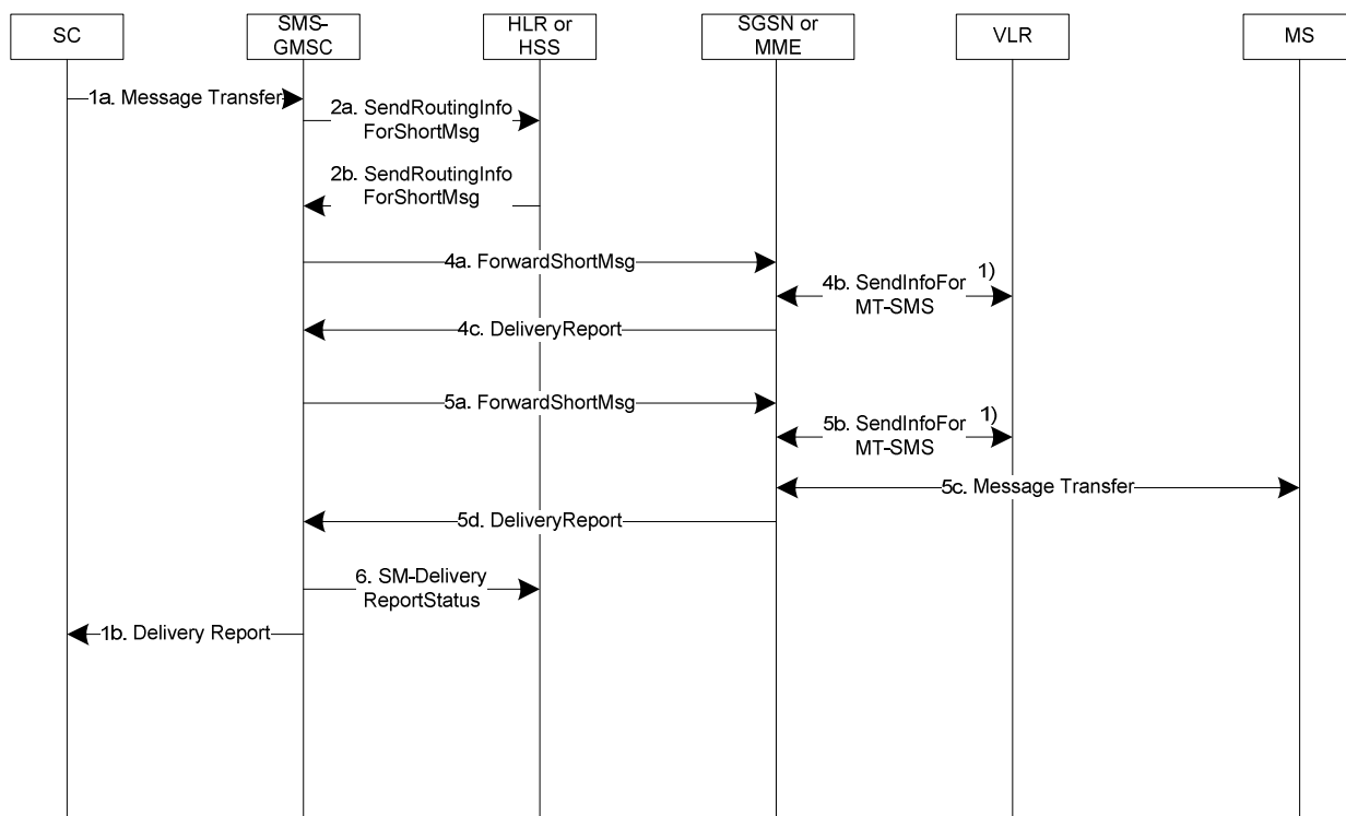
Figure 17a): Successful short message transfer attempt via the SGSN or MME, with short message retransmission by the SMS-GMSC at the time requested by the SGSN or MME
