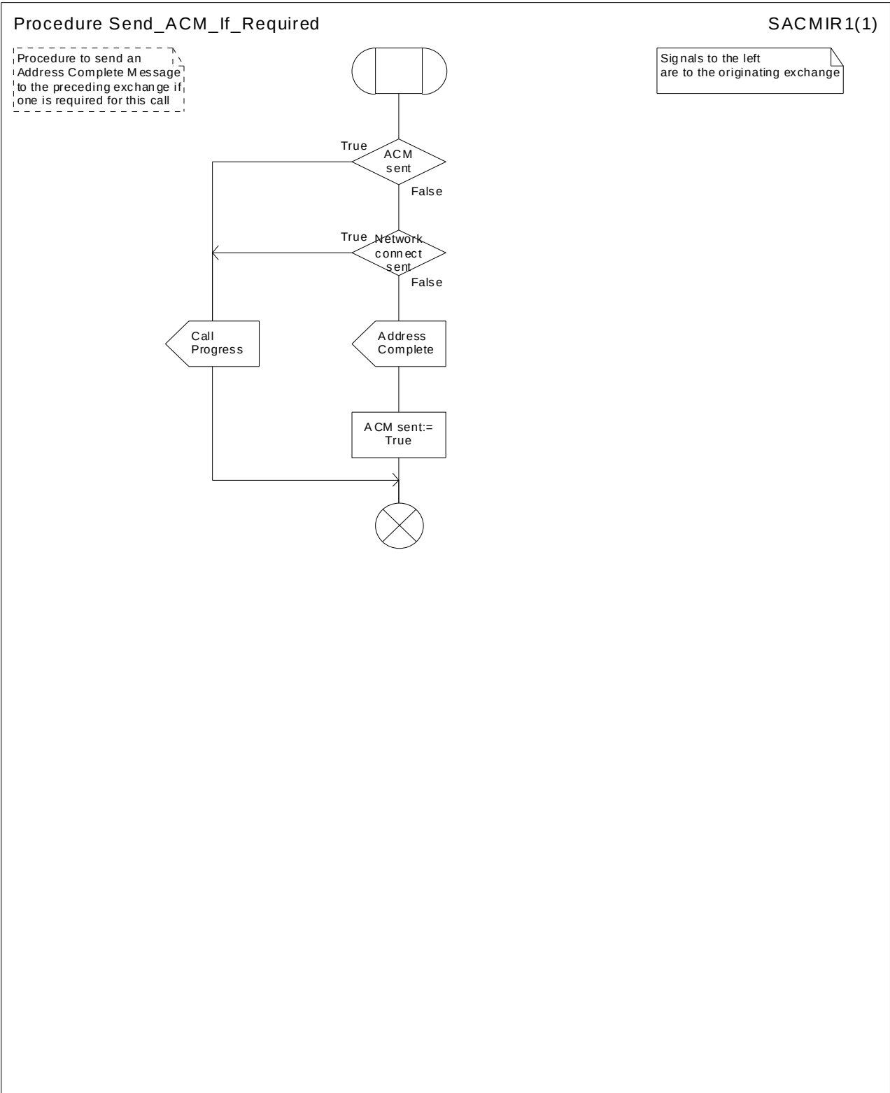
Figure 38: Procedure Send_ACM_If_Required
