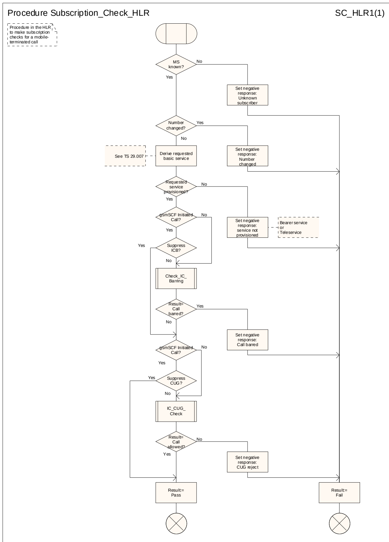
Figure 46: Procedure Subscription_Check_HLR
