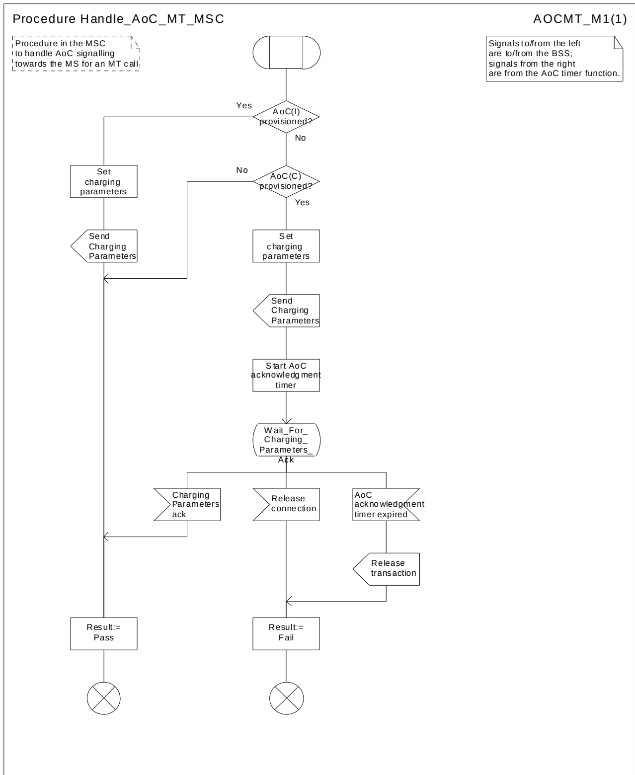
Figure 74: Procedure Handle_AoC_MT_MSC
