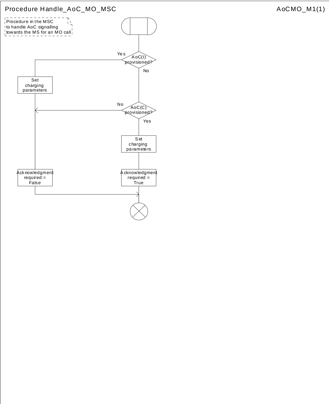
Figure 17: Procedure Handle_AoC_MO_MSC
