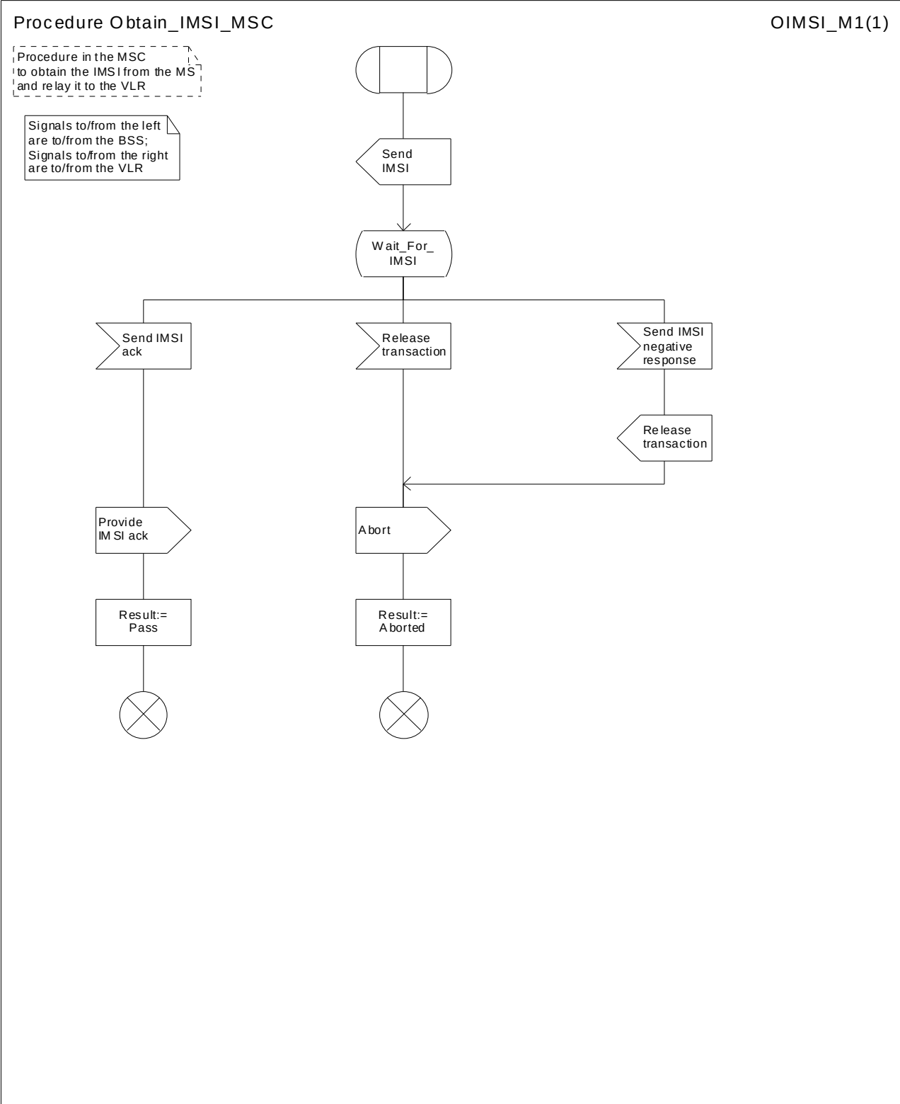
Figure 9: Procedure Obtain_IMSI_MSC
