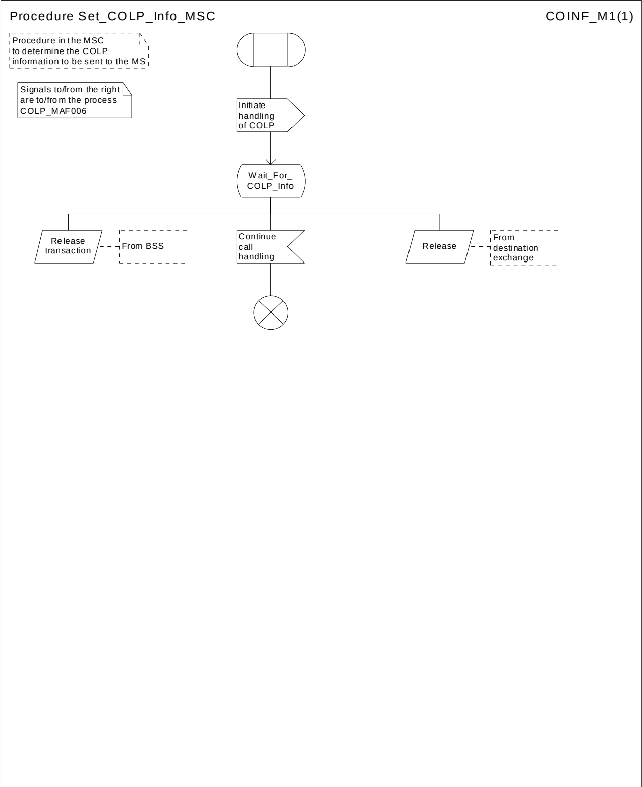
Figure 16: Procedure Set_COLP_Info_MSC
