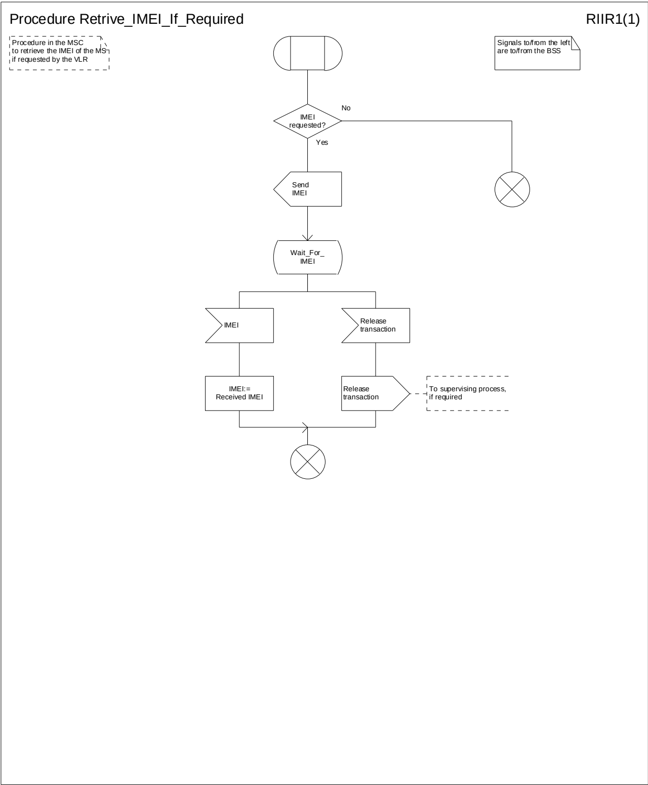
Figure 66bis: Procedure Retrive_IMEI_If_Required
