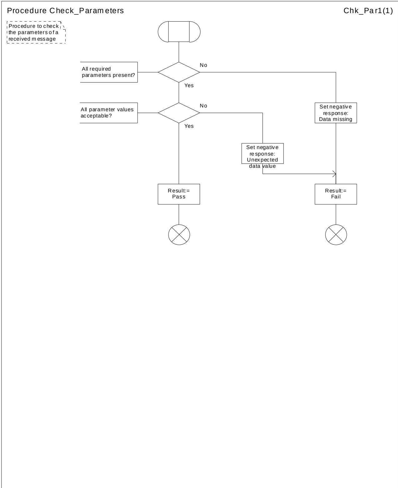
Figure 45: Procedure Check_Parameters
