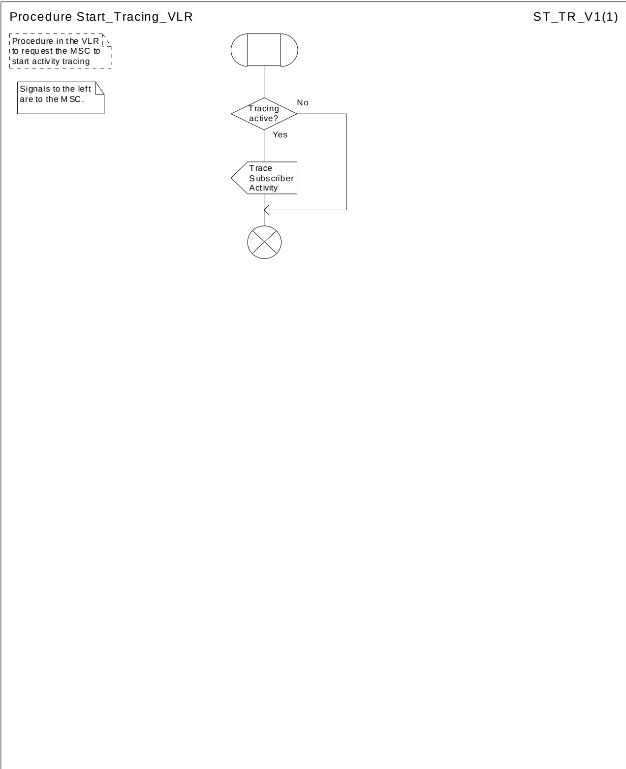
Figure 7.1.2.8: Procedure Start_Tracing_VLR
