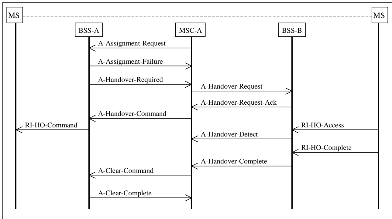
Figure 40: Example of a Directed Retry Intra-MSA Handover Procedure
