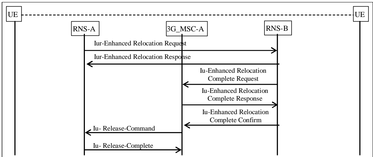
Figure 11a: Basic intra-3G_MSC Enhanced SRNS Relocation Procedure
