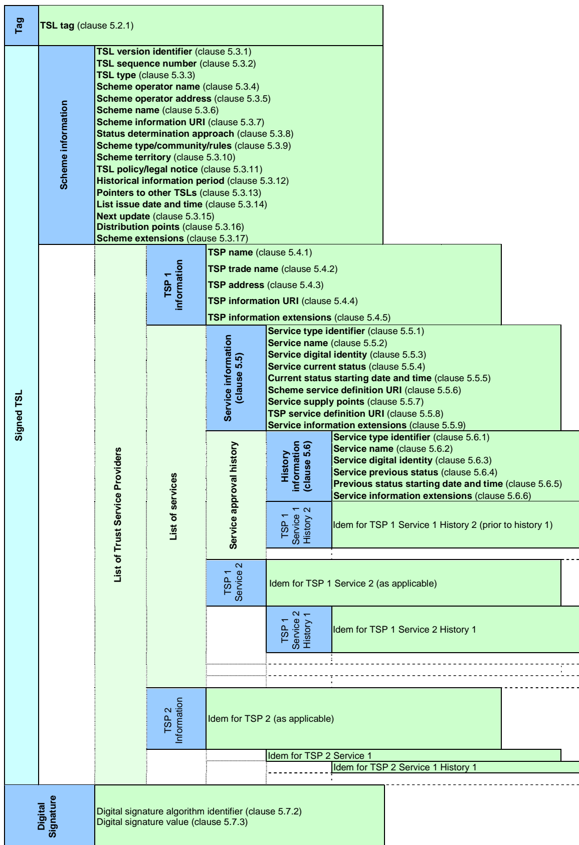
Figure 1: Logical model of the trusted list
