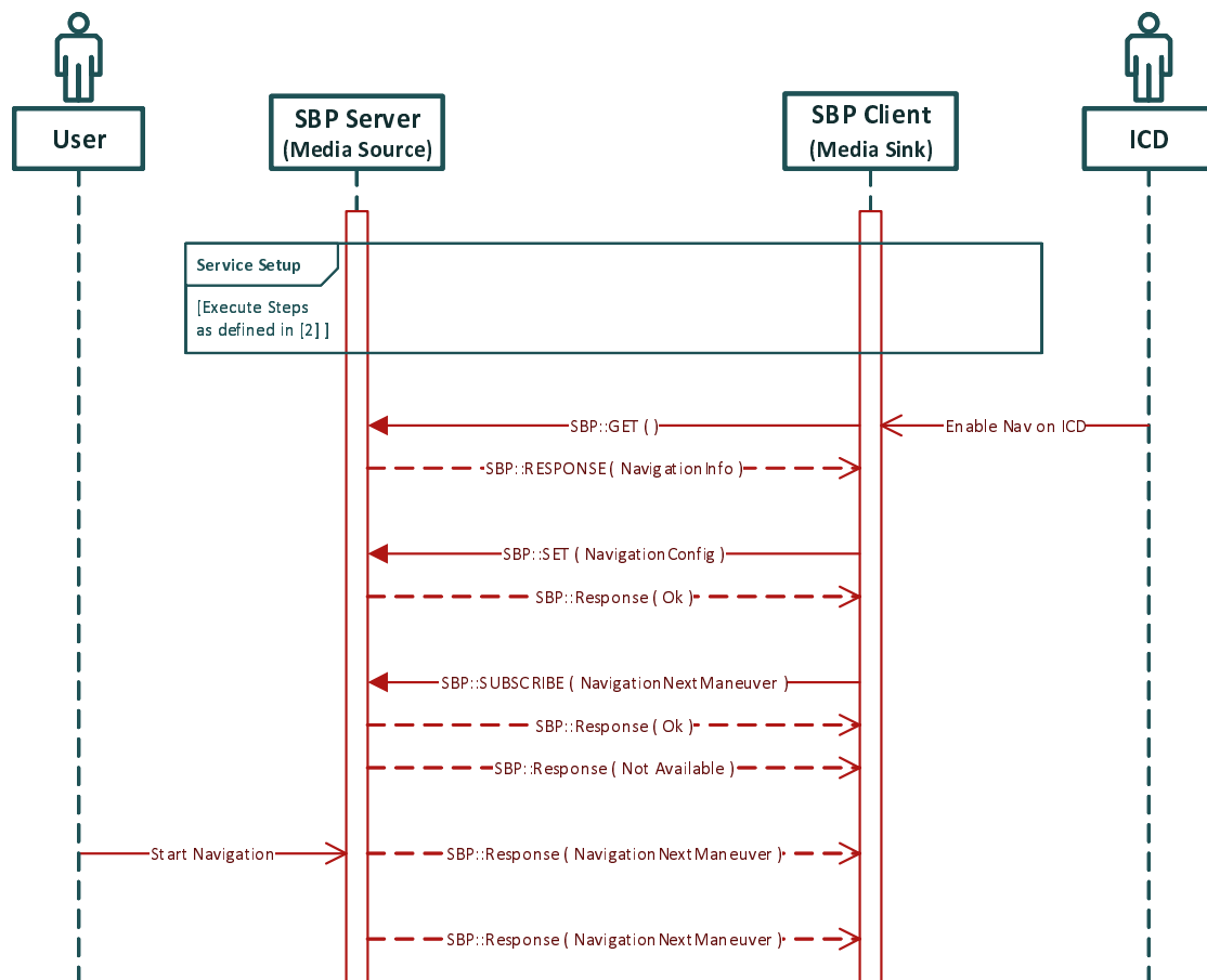
Figure 2: Message Sequence Diagram - Turn-by-Turn Navigation
