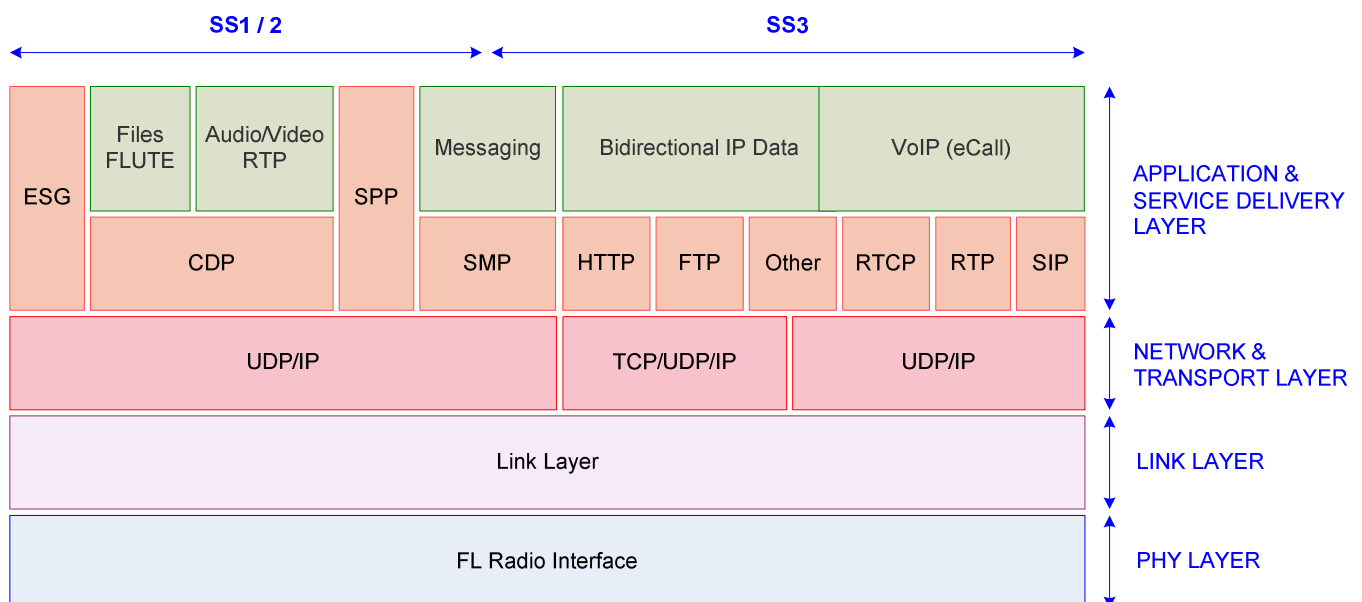
Figure 7.1: Generalized protocol stack for the Forward link
