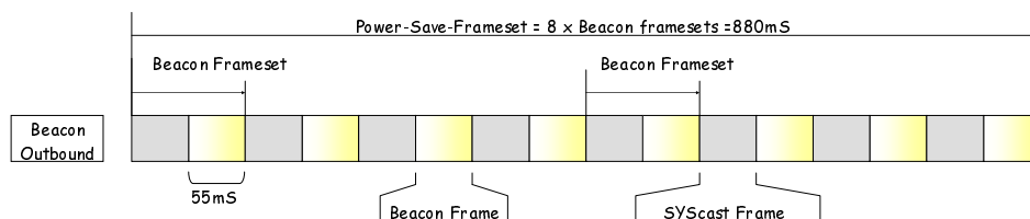
Figure 12.5: Beacon frames and Framesets
