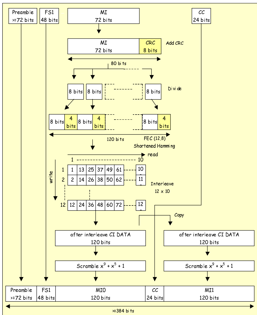
Figure 11.8: Message coding
