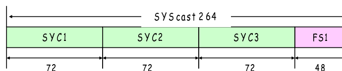
Figure 4.11: SYScast Frame
