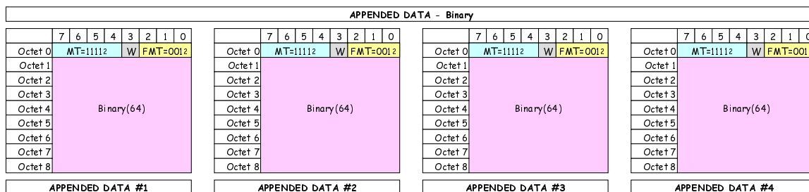
Figure 5.10: Appended_Data (Binary)
