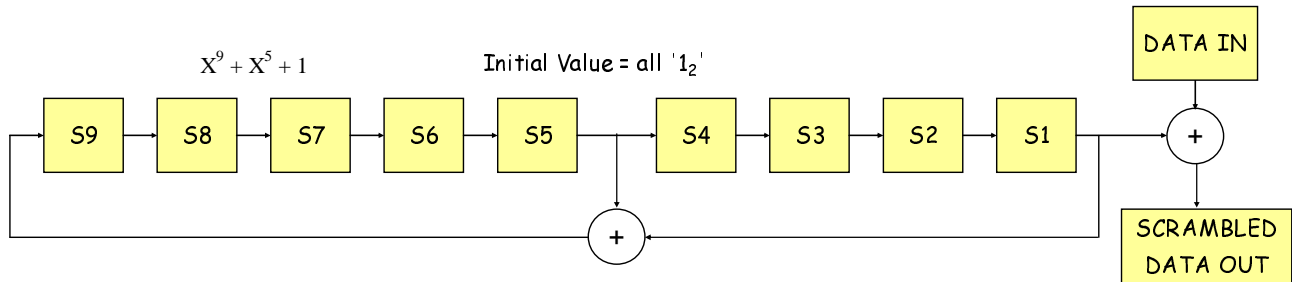
Figure 7.1: Scrambling format
