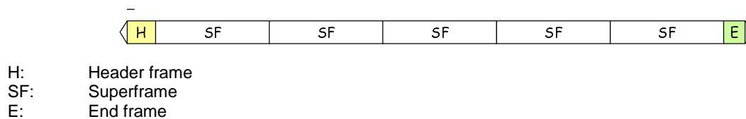
Figure 4.12: Voice or Data Payload continuous transmission
