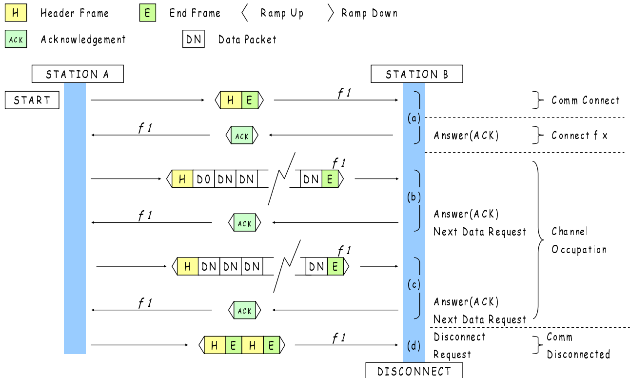
Figure 9.3: Packet exchanges
