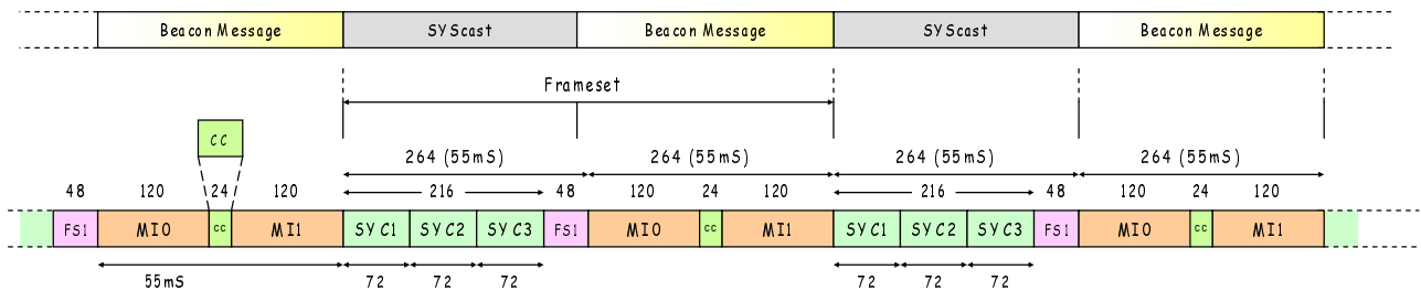
Figure 12.6: Beacon Channel Downlink
