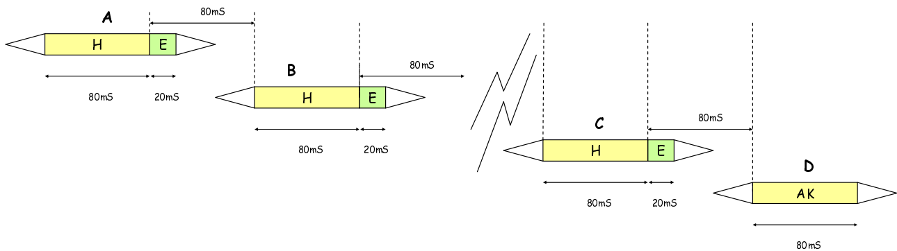
Figure 10.21: Co-Channel BS/MS timing
