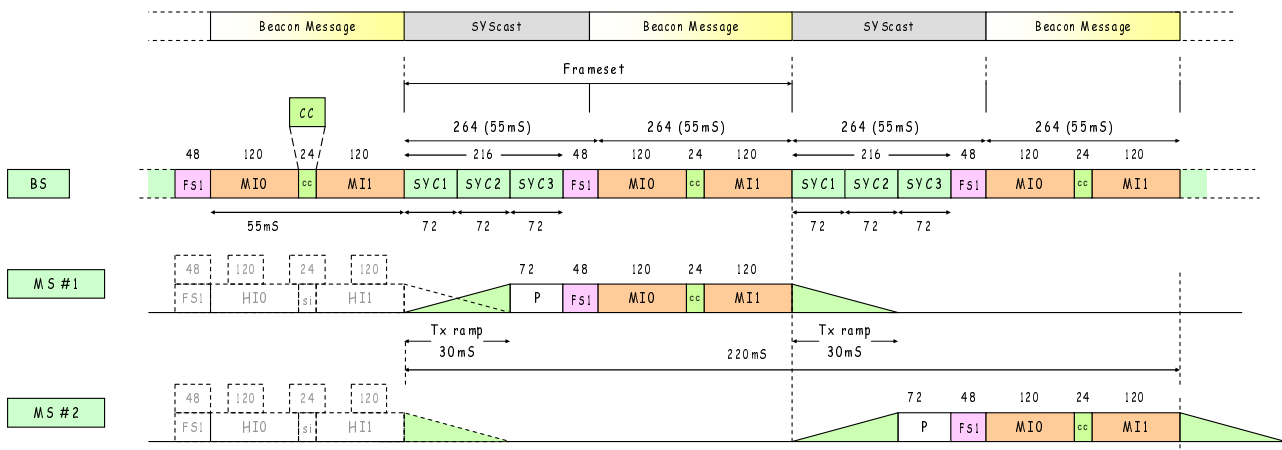
Figure 12.4: Beacon Timing
