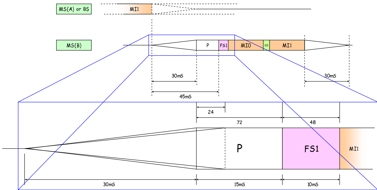
Figure 12.1 : Preamble Timing
