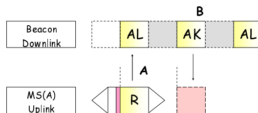
Figure 12.20: Registration Exchange
