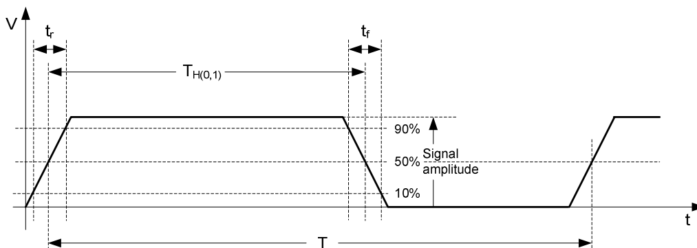
Figure 8.2: S1 waveform
