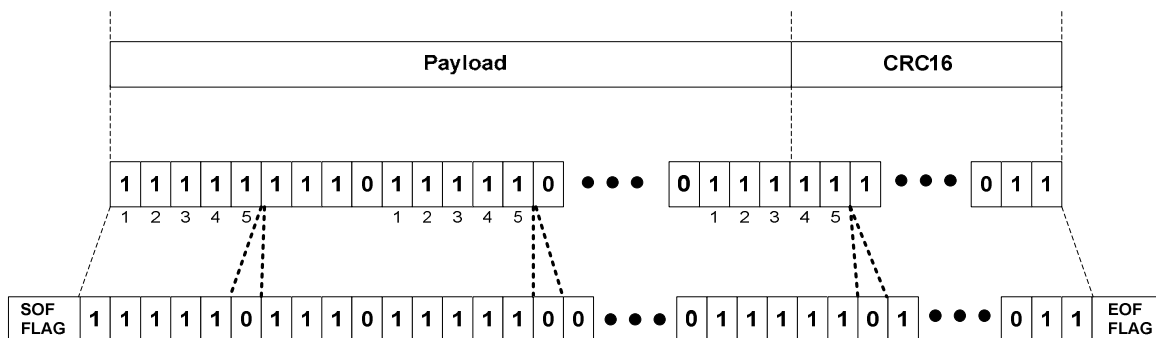
Figure 9.4: Bit stuffing
