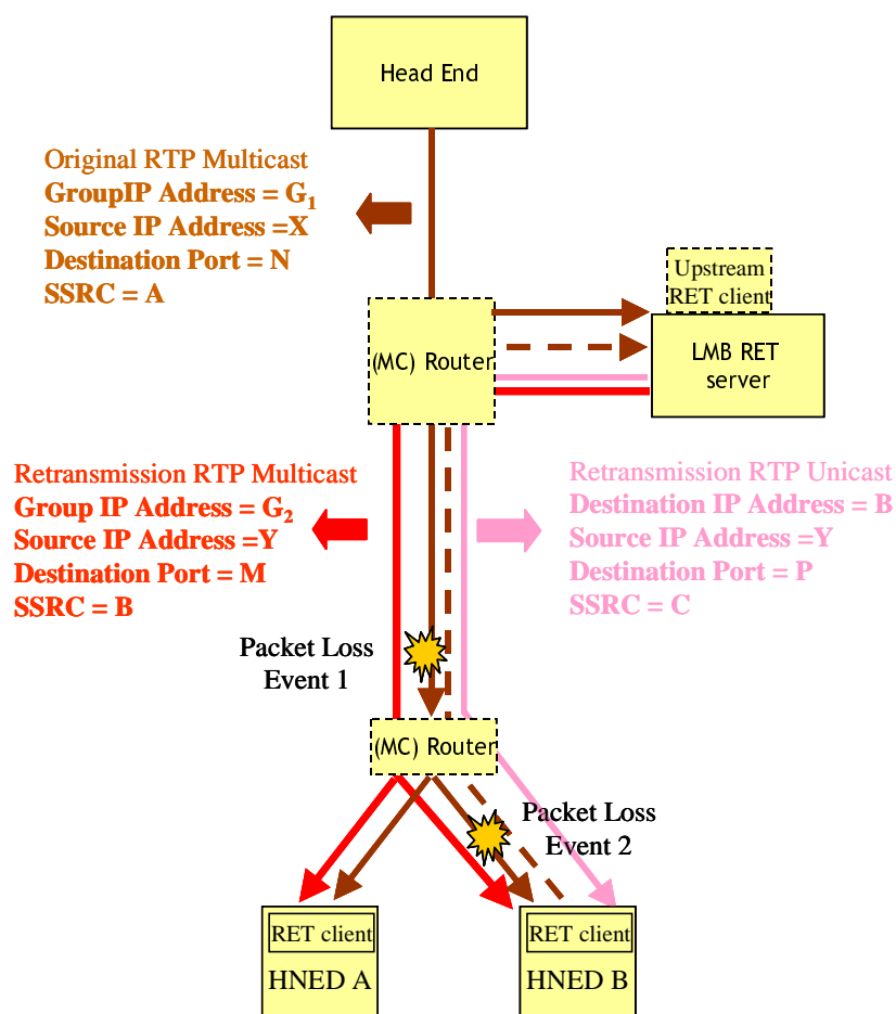
Figure 4.1: Architecture example for a RET-enabled LMB service
