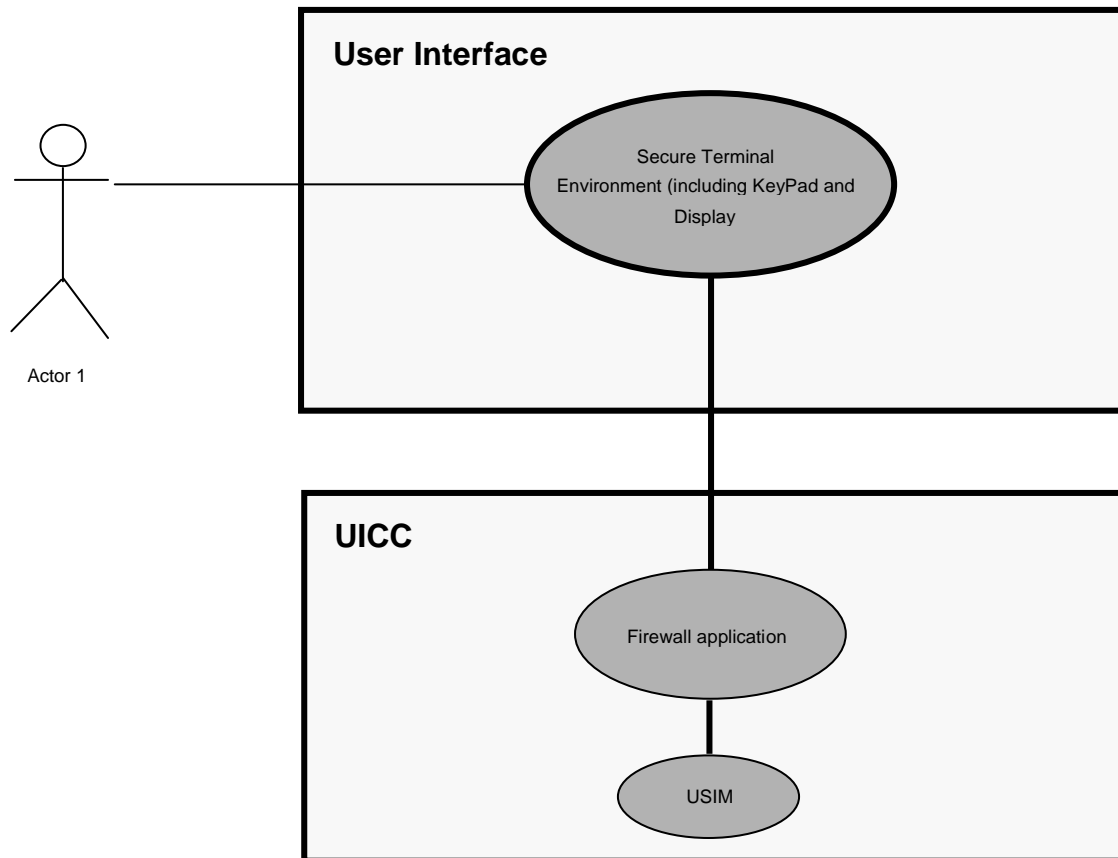
Figure 2: User Interfaces
