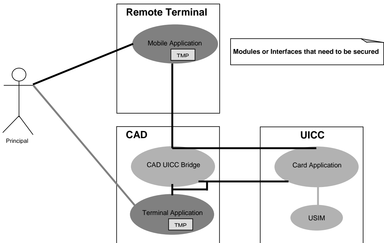
Figure 4: Distributed application
