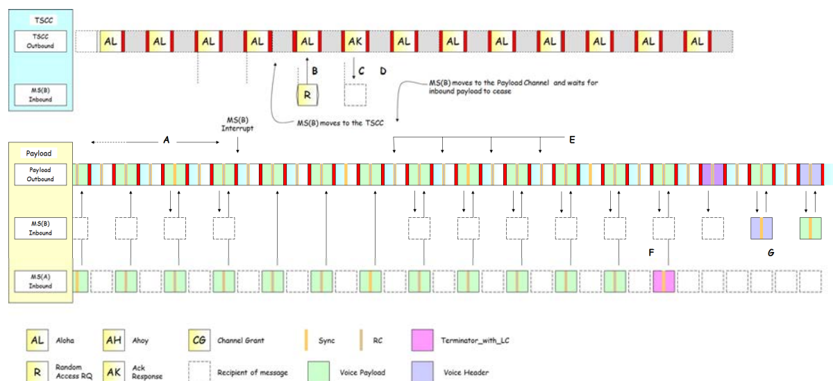
Figure 6.37: Payload Interrupt
