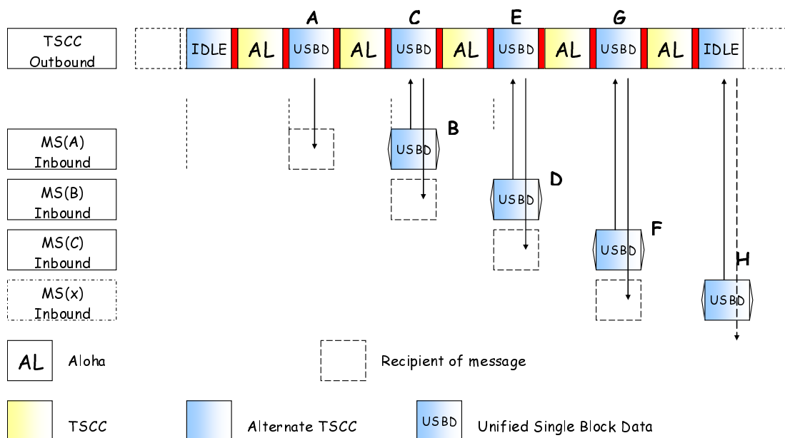
Figure 6.60: Example of Unified Single Block Data Polling Service on TSCCAS using Aligned Timing (Response Delay=00 2 )
