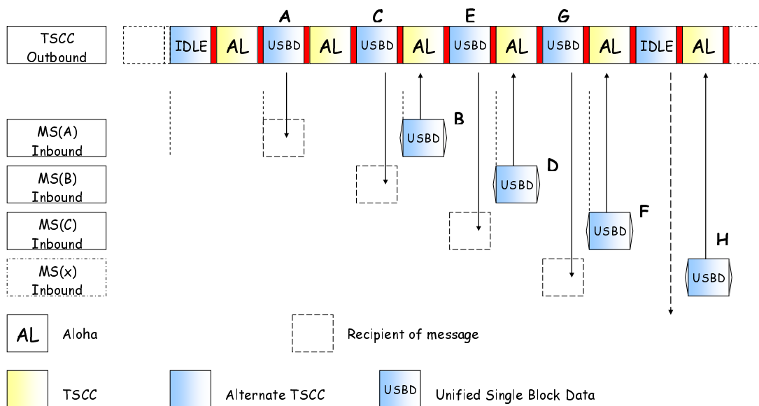
Figure 6.61: Example of Unified Single Block Data Polling Service on TSCCAS using Offset Timing (Response Delay = 00_2 )
