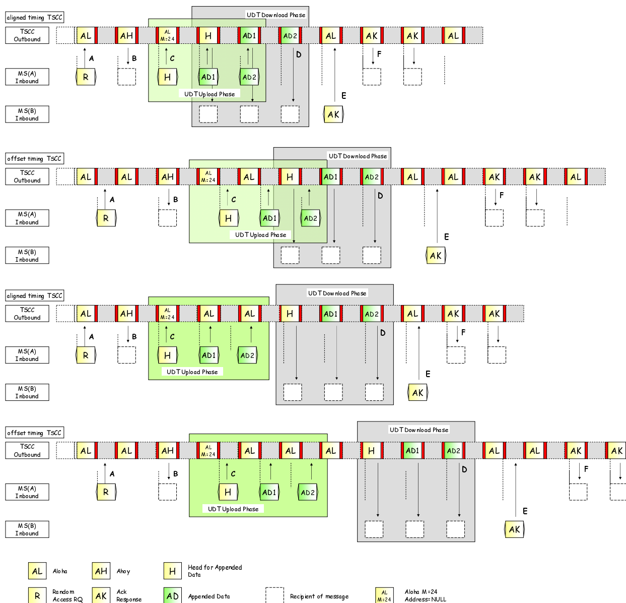
Figure 6.50: More Examples of a UDT Short Data Message transfer
