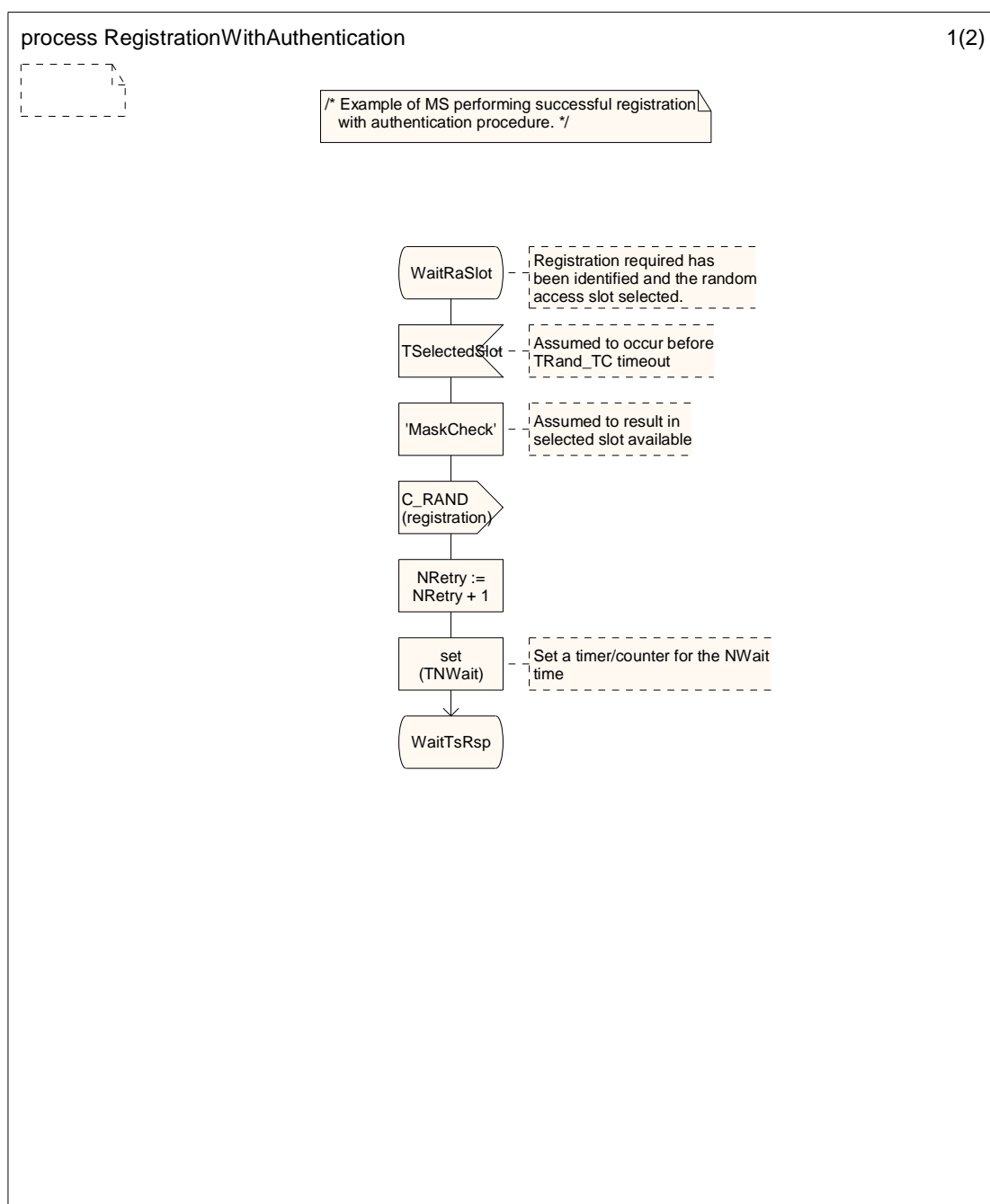
Figure 6.22 (sheet 1 of 2): Registration with Authentication SDL
