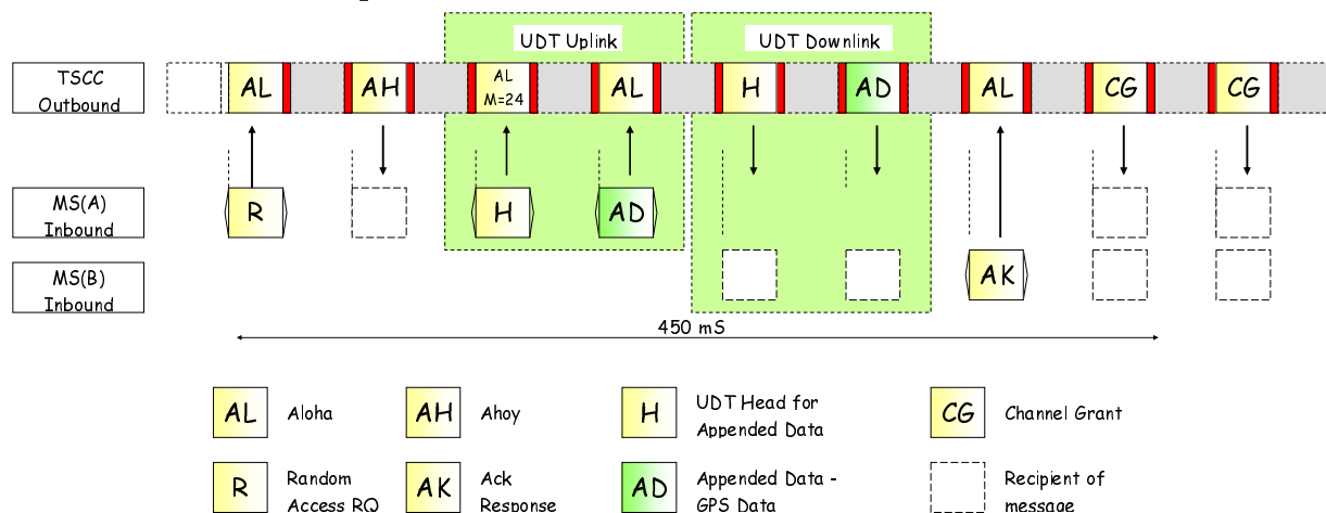
Figure 6.37: UDT mechanism carrying supplementary data
