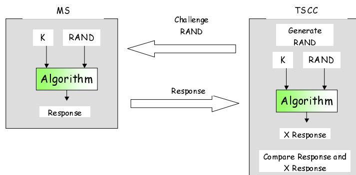
Figure 6.25: Challenge and Response Authentication
