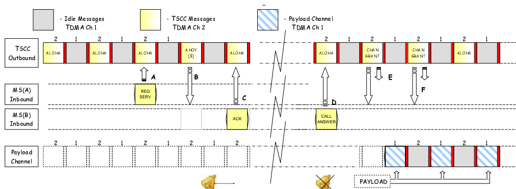
Figure 6.39: Call Answer Mechanism for FOACSU
