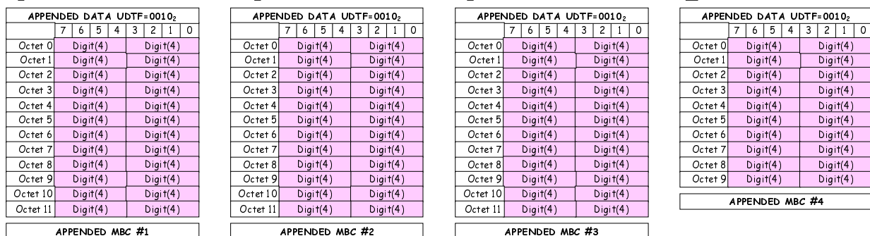
Figure B.10: Unified Data Transport Format (BCD) 66 digits to 92 digits
