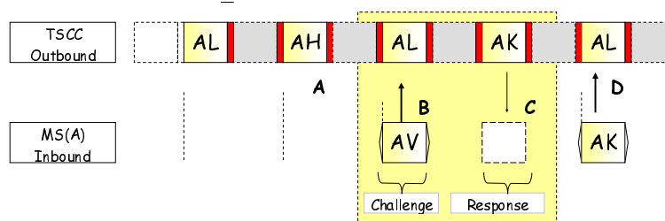
Figure 6.27: MS Stun/Revive with Authentication
