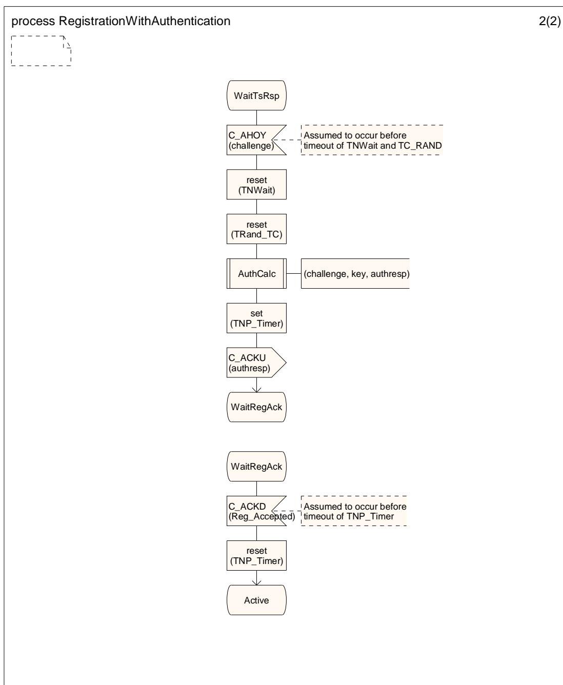
Figure 6.23 (sheet 2 of 2): Registration with Authentication SDL
