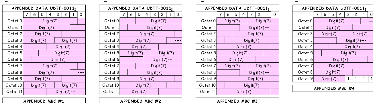
Figure B.14: Unified Data Transport Format (ISO 7 bit) 39 text symbols to 52 text symbols
