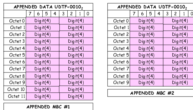
Figure B.8: Unified Data Transport Format (BCD) 21 digits to 44 digits
