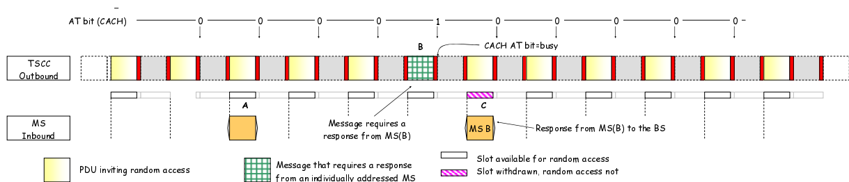
Figure 6.5: Withdrawn Slots Example
