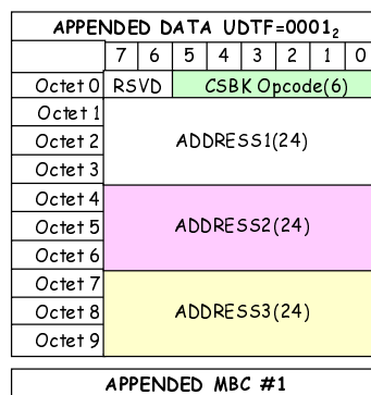
Figure B.6: Appended data Address Format
