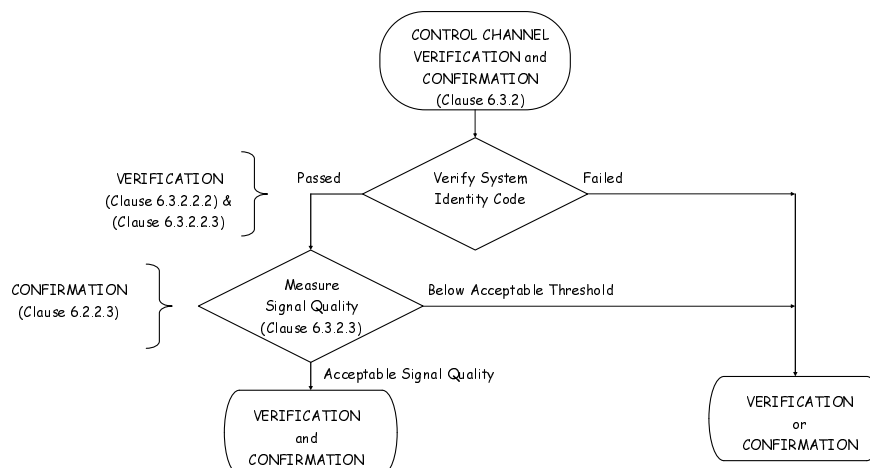
Figure 6.14: Verification and Confirmation Steps
