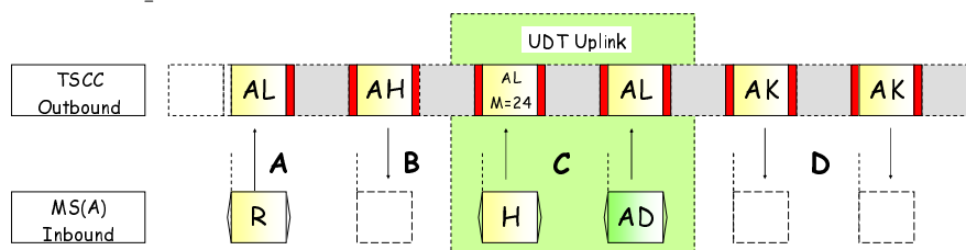
Figure 6.49: Example of a Call Diversion Call
