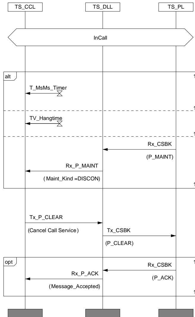
Figure 6.43: Voice Call Termination MSC
