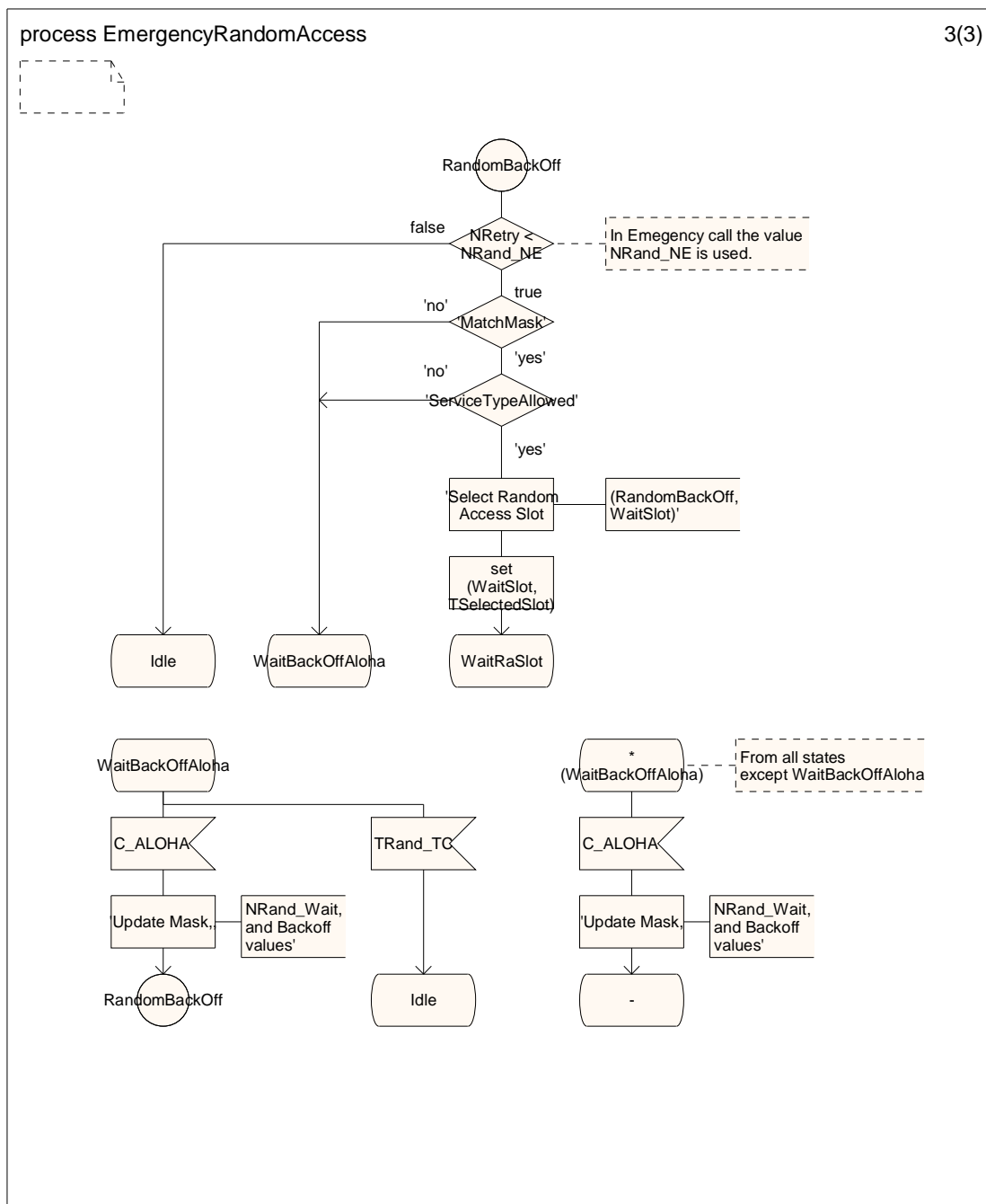
Figure 6.13 (sheet 3 of 3): Emergency Random Access Procedure SDL
