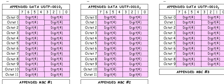
Figure B.9: Unified Data Transport Format (BCD) 45 digits to 65 digits
