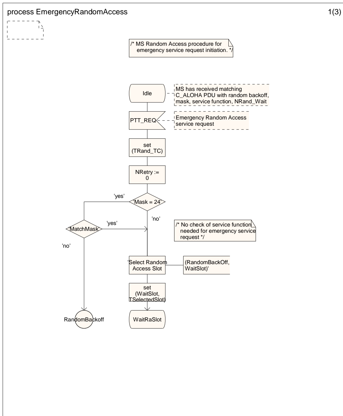
Figure 6.11 (sheet 1 of 3): Emergency Random Access Procedure SDL
