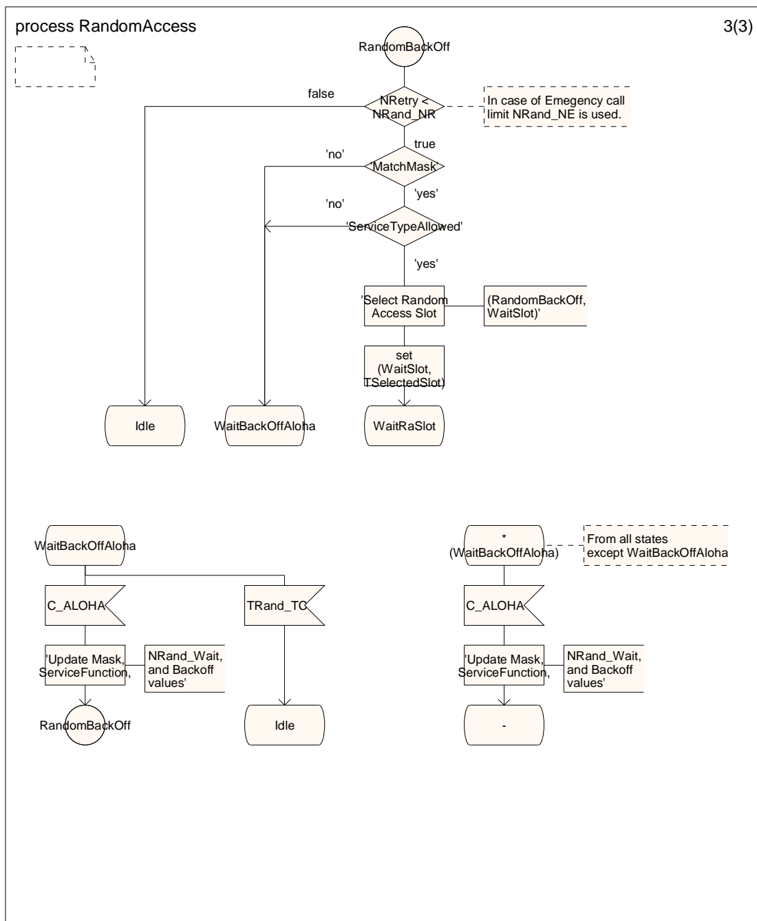
Figure 6.10 (sheet 3 of 3): Random Access Procedure SDL
