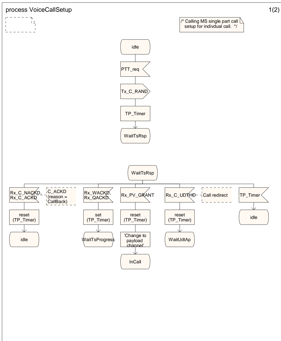
Figure 6.40 (sheet 1 of 2): Single part OACSU voice call setup SDL
