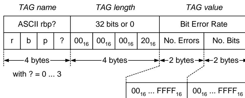
Figure 6.28: Bit error rate of MSC stream &lt;n&gt;
