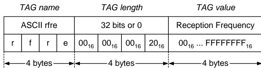
Figure 6.9: Reception frequency
