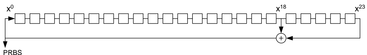
Figure 7.1: Shift register for PRBS G_{23}(x) generation
