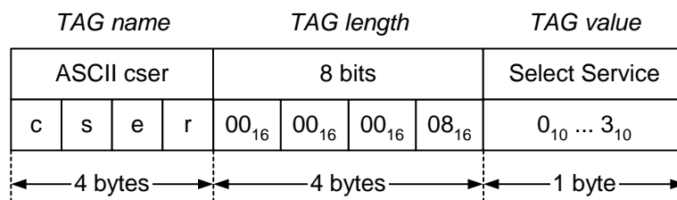
Figure 6.38: Select service
