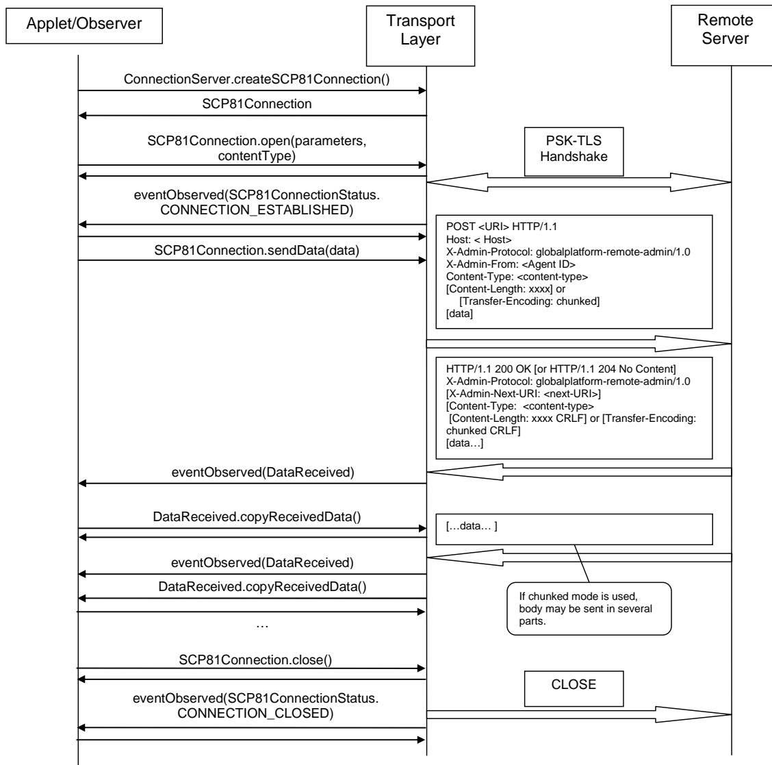
Figure 5: SCP81Connection sequence diagram
