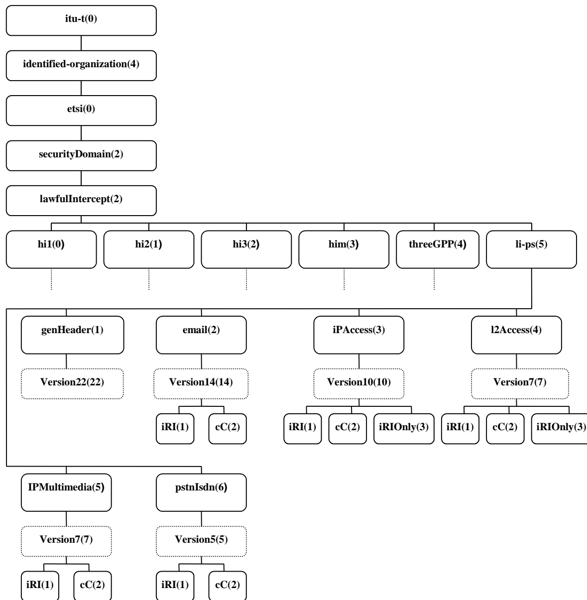
Figure A.1: Object identifier tree
