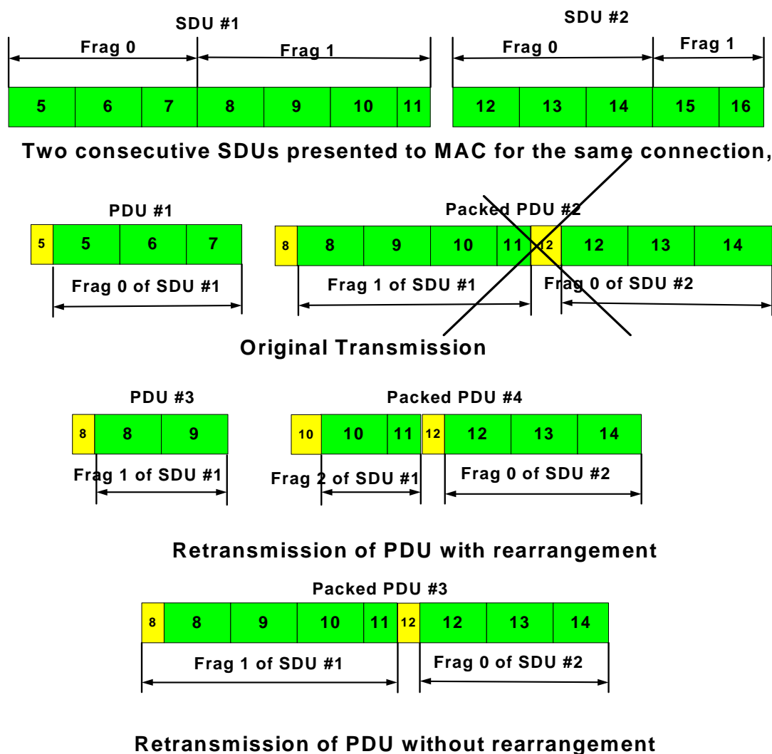
Figure 4: Block usage examples for ARQ transmissions and retransmissions
