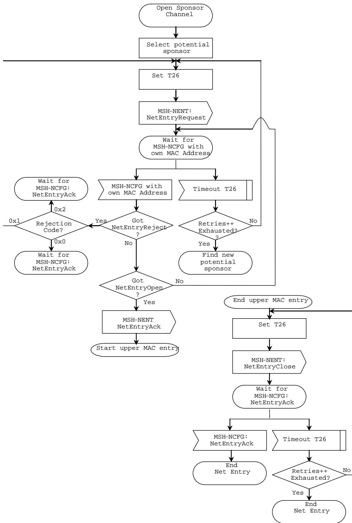
Figure 11: Synchronization and network entry - new node II
