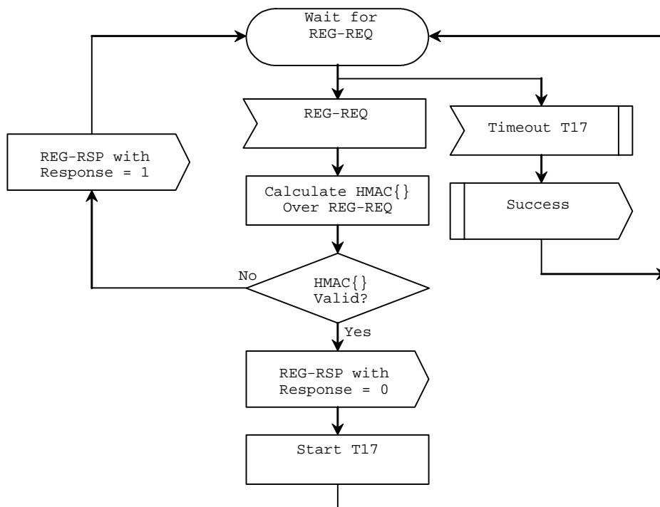
Figure 14: Registration - registration node
