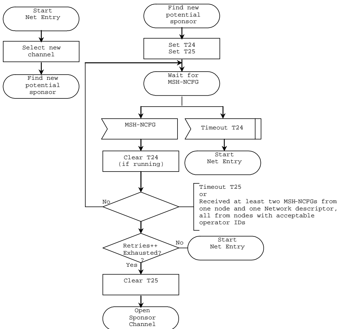
Figure 10: Synchronization and network entry - new node I
