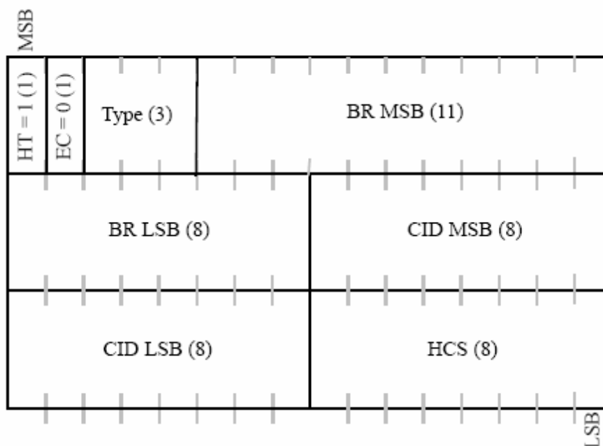
Figure 2: Bandwidth request header format
