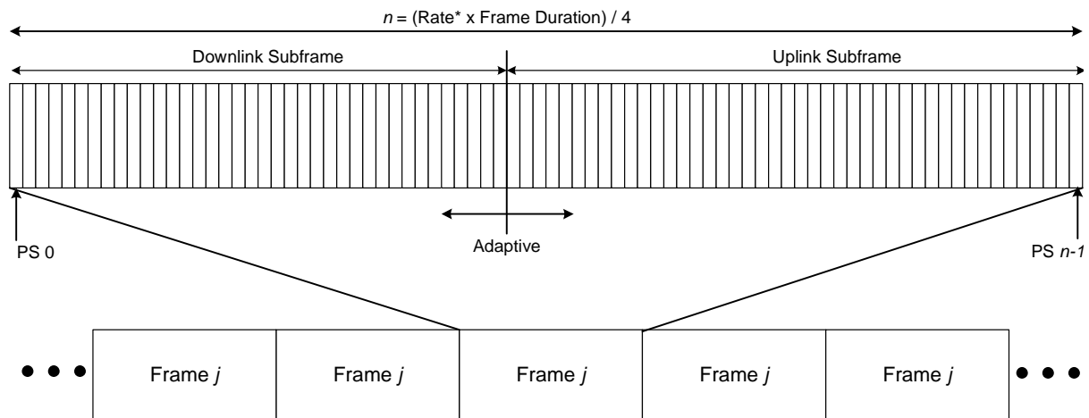
Figure 18: TDD frame structure
