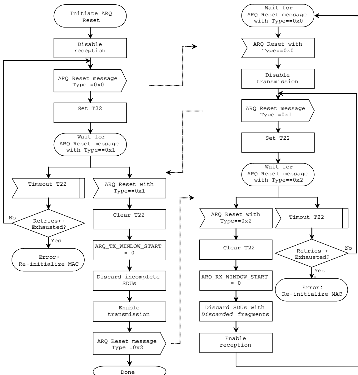
Figure 8: Transmitter initiated ARQ Reset
