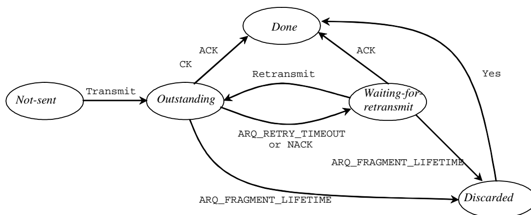
Figure 5: Transmitter ARQ state machine
