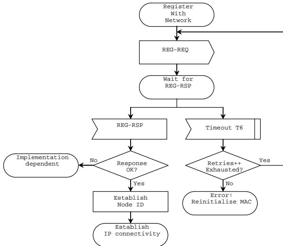
Figure 13: Registration - candidate node
