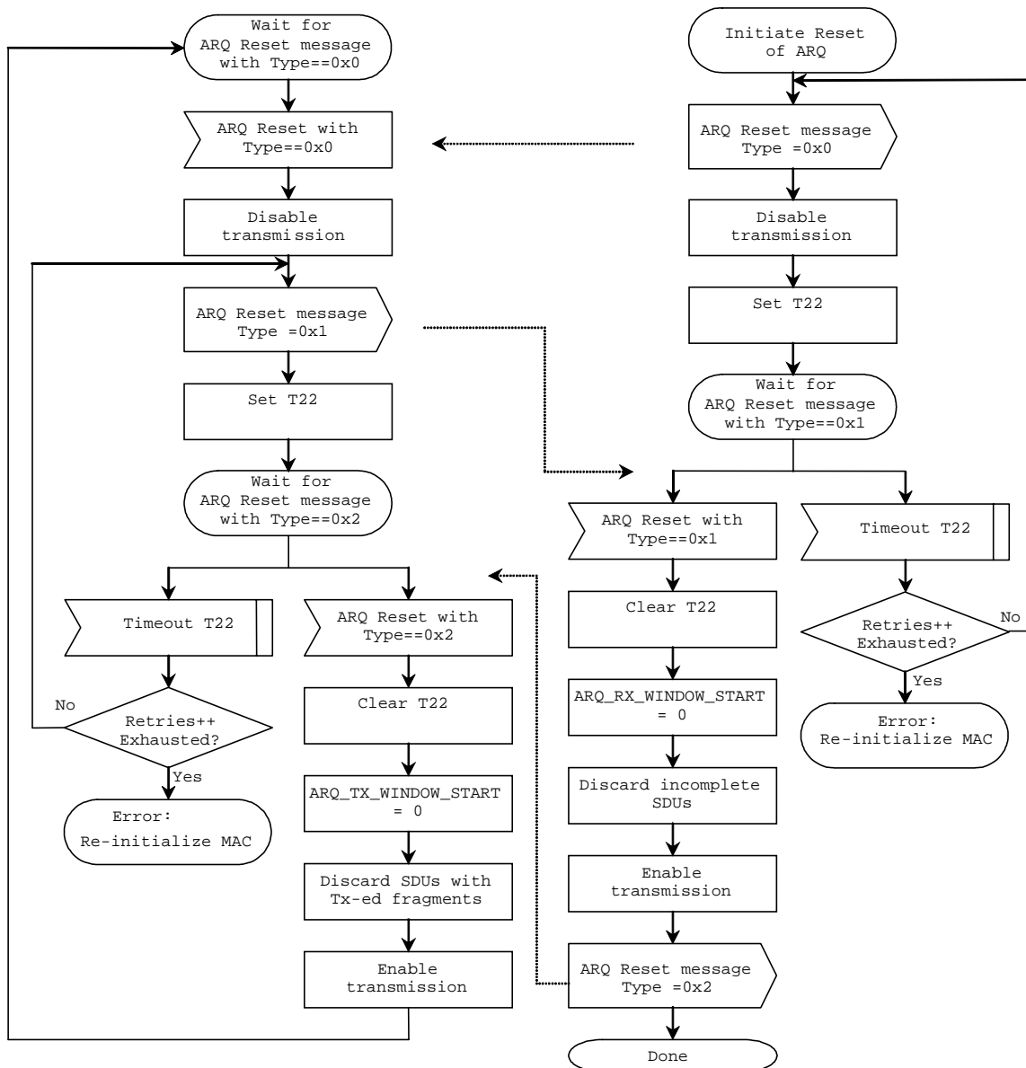
Figure 7: Receiver initiated ARQ Reset
