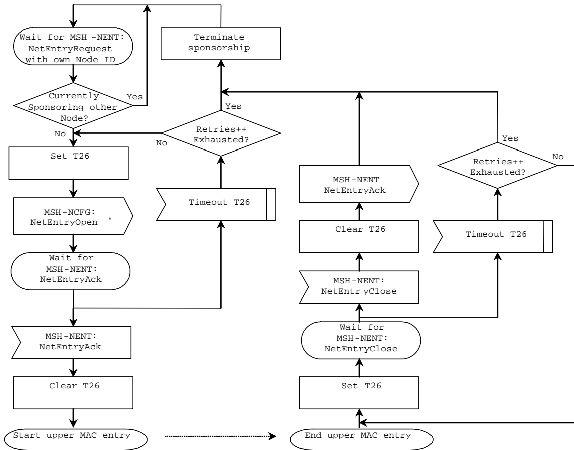
Figure 12: Synchronization and network entry - sponsor node
