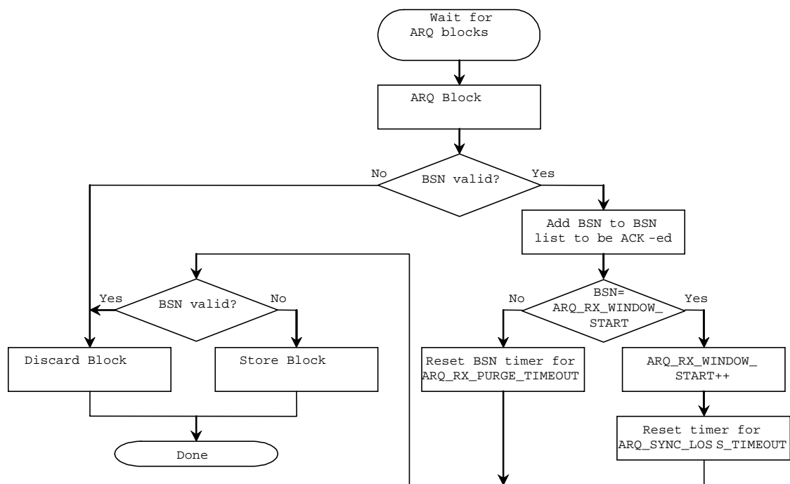
Figure 6: ARQ block reception
