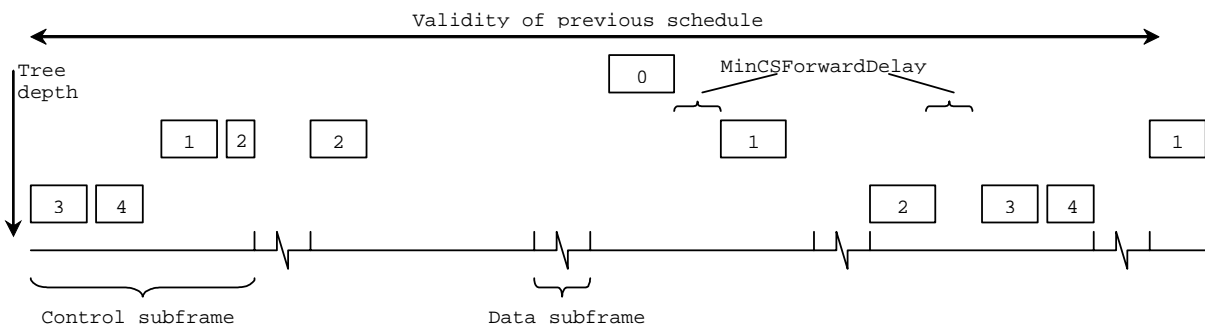
Figure 17: MSH-CSCH schedule validity
