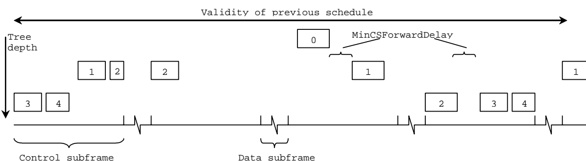
Figure 17: MSH-CSCF schedule validity
