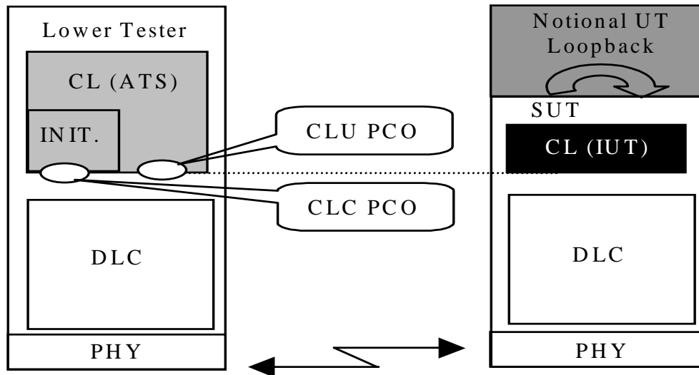
Figure 1: Test architecture for Packet CL-Ethernet SSCS
