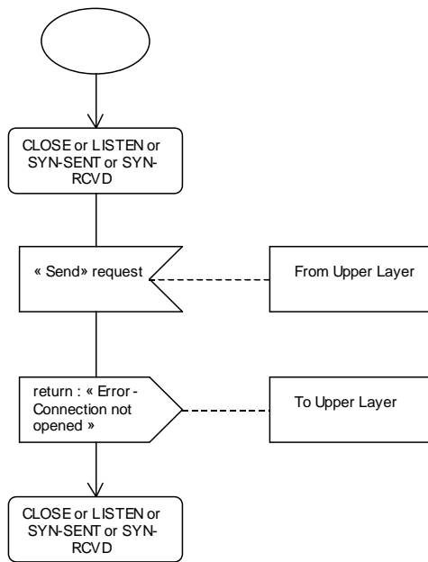
Figure 22: Send request in CLOSE, LISTEN, SYN-SENT or SYN-RCVD state
