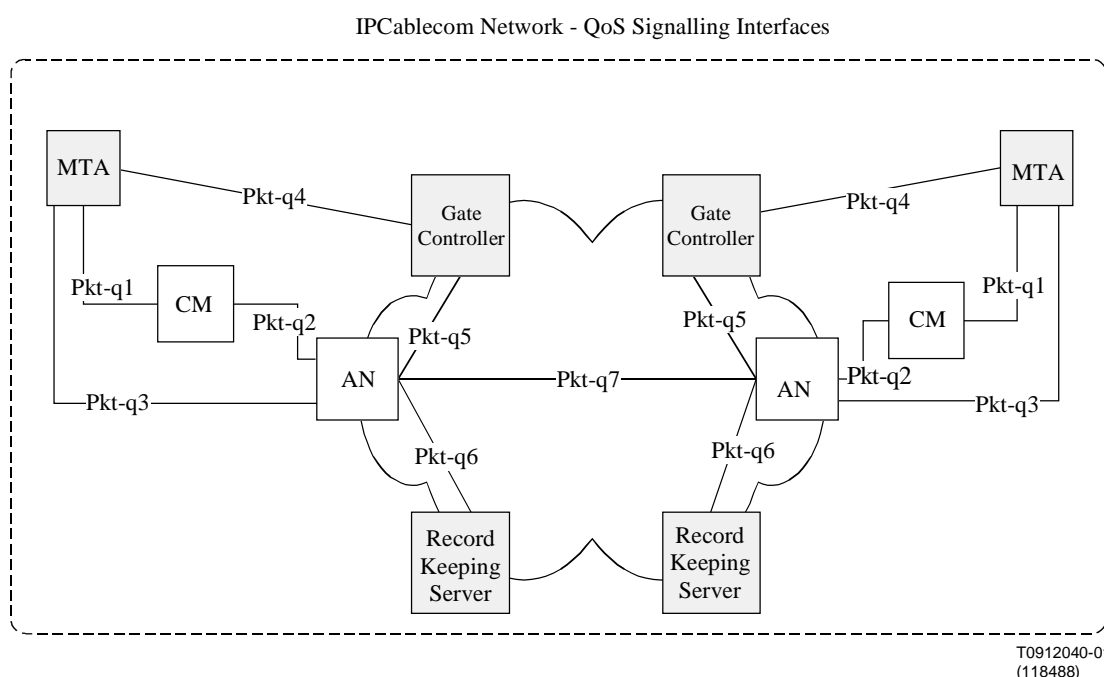
Figure 11: IPcablecom QoS Signalling Interfaces
