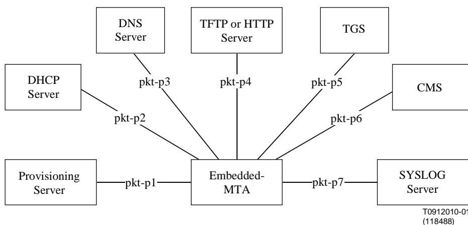
Figure 8: IPCablecom Provisioning Interfaces
