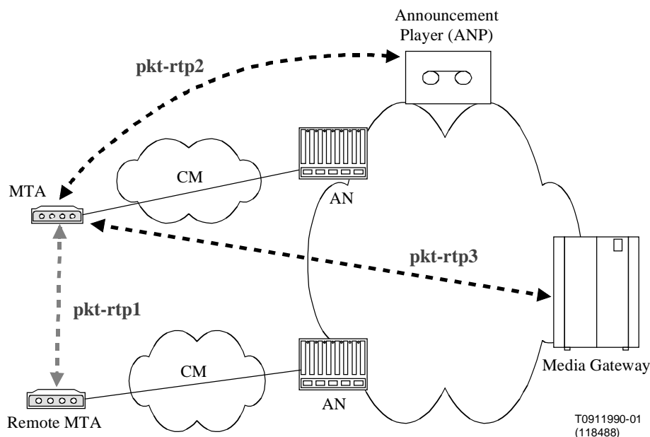
Figure 6: RTP Media Stream Flows in an IP-Cablecom Network
