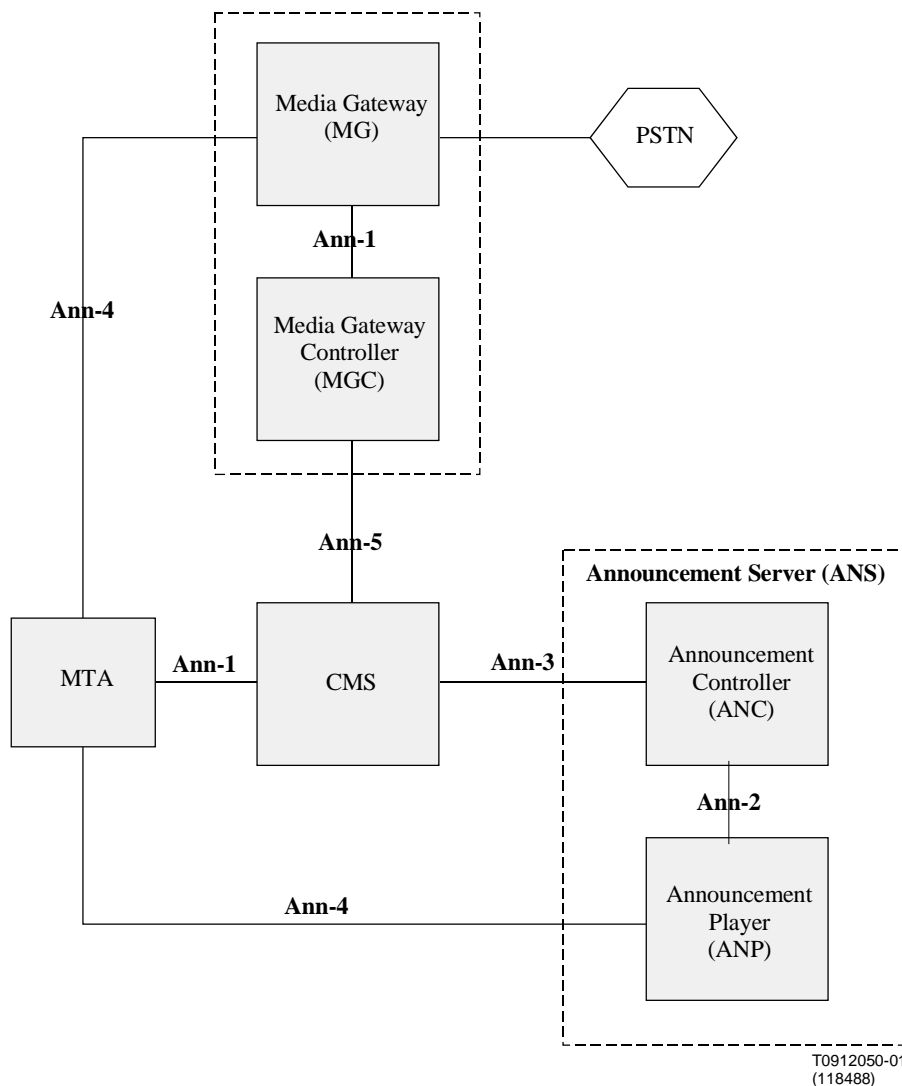
Figure 12: Announcement Services Components and Interfaces
