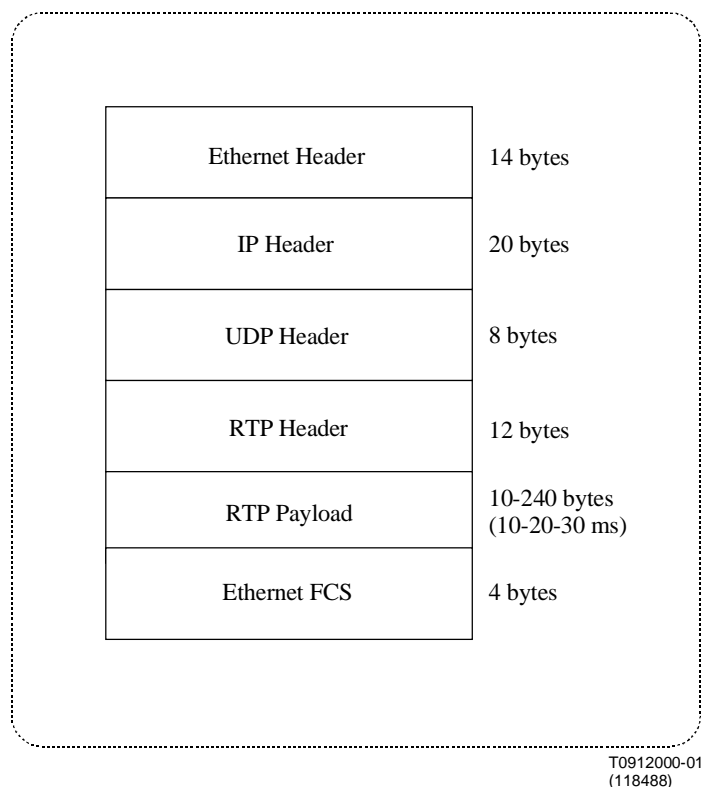
Figure 7: RTP Packet Format
