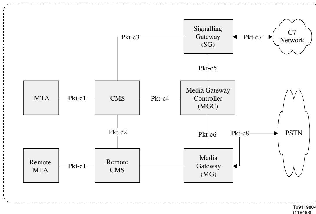
Figure 5: Call Signalling Interfaces
