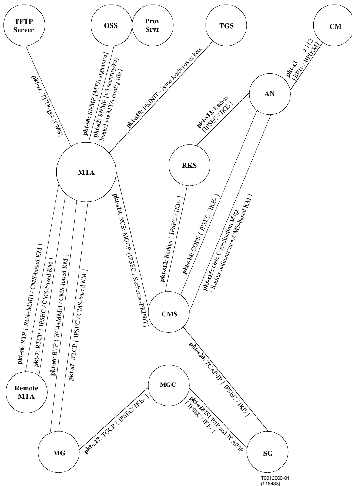
Figure 13: IPCablecom Security Interfaces
