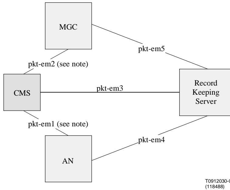
Figure 9: Representative Event Messages Architecture
