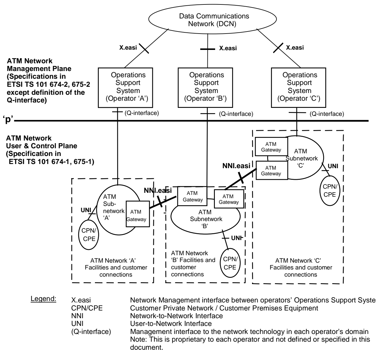
Figure 1: Technical scope and the interfaces
