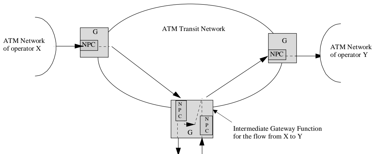
Figure 2: Location of NPC functions in the ATM Transit Network
