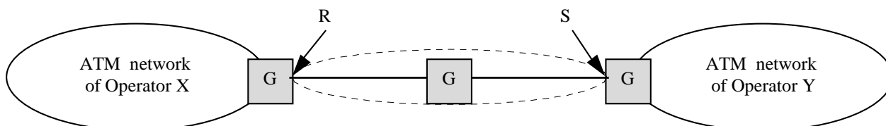
Figure 3: Scope of performance and availability targets for the ATM transit portion
