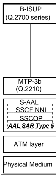
Figure 4: Protocol stack at the NNI.easi interface
