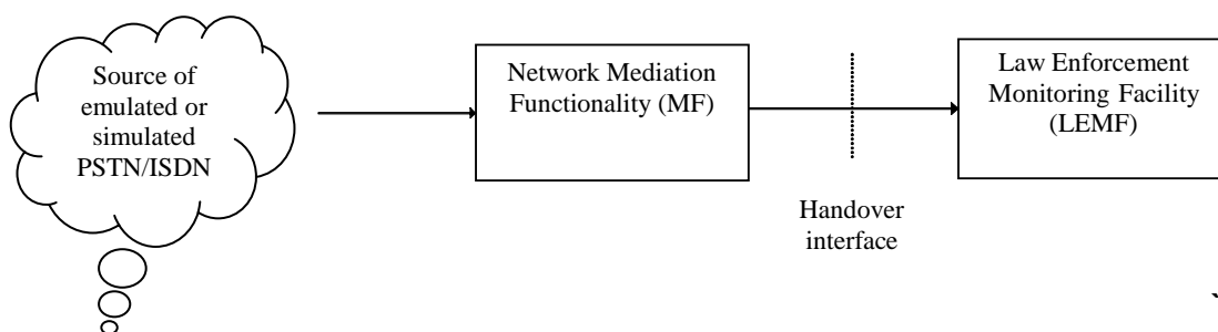
Figure A.10.1: High level functional architecture for PSTN/ISDN emulation and simulation services
