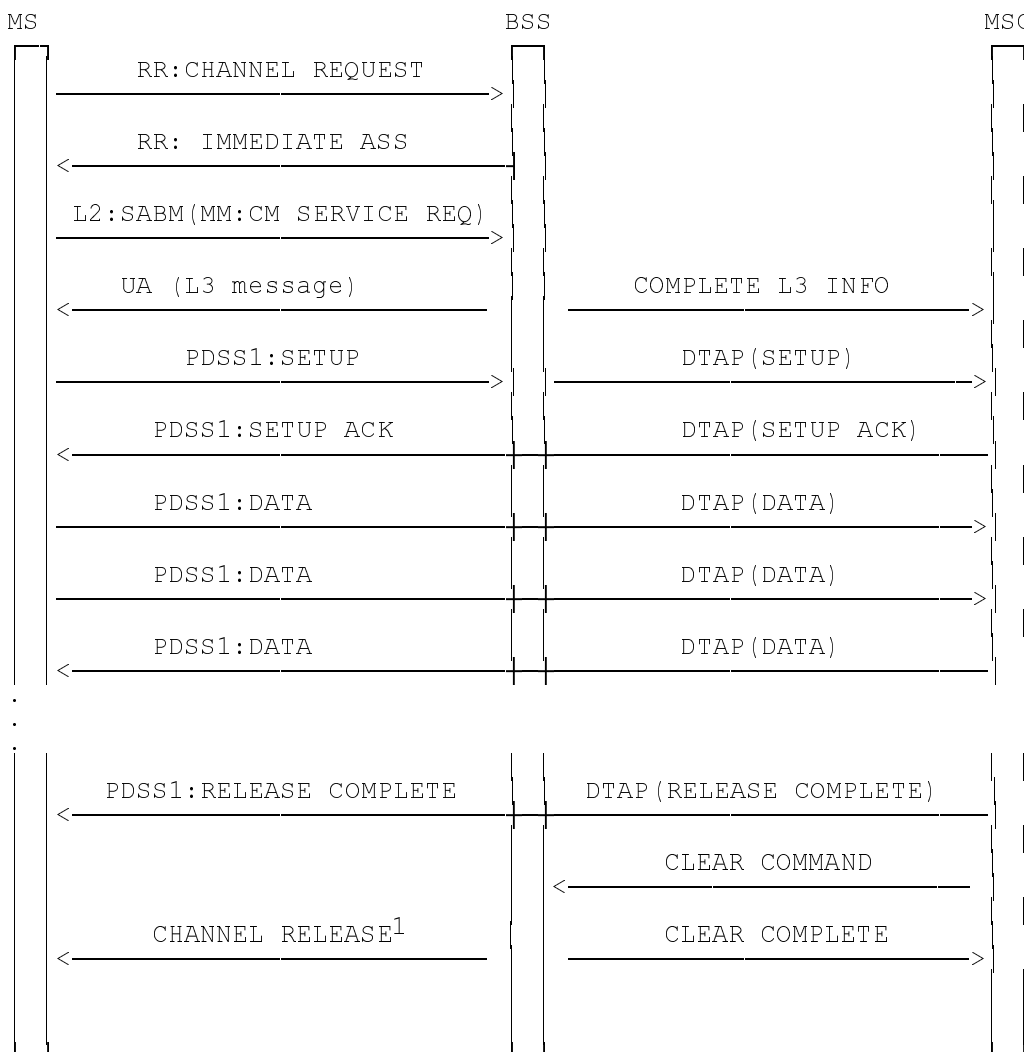
Figure 1: Signalling flow for mobile originating PDSS1 (starting in idle mode, release by MSC)
