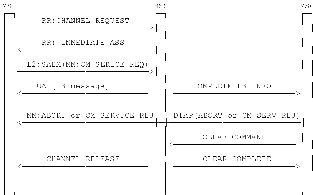
Figure 4: Signalling flow for PDSS1 (rejection of PDSS1-service)
