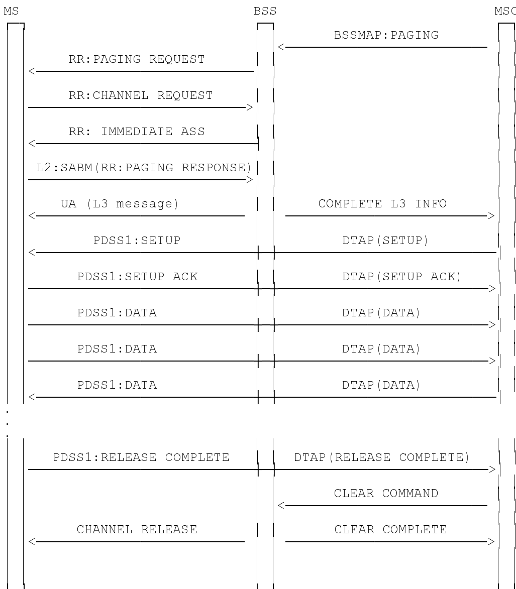
Figure 2: Signalling flow for mobile terminating PDSS1 (from idle mode, release by mobile station)
