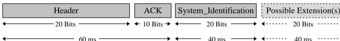
Figure 18: General Construction of an IS_ACK Message
