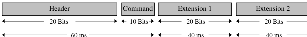
Figure 13: Example for IS Message with two IS_Extension_Blocks
