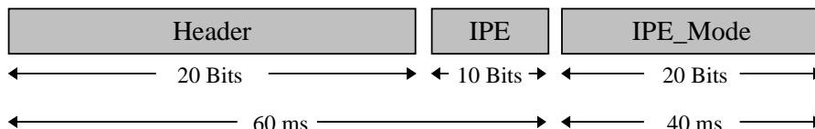
Figure 19: General Construction of an IS_IPE Message
