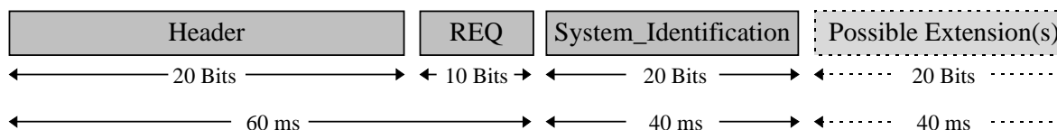
Figure 17: General Construction of an IS_REQ Message
