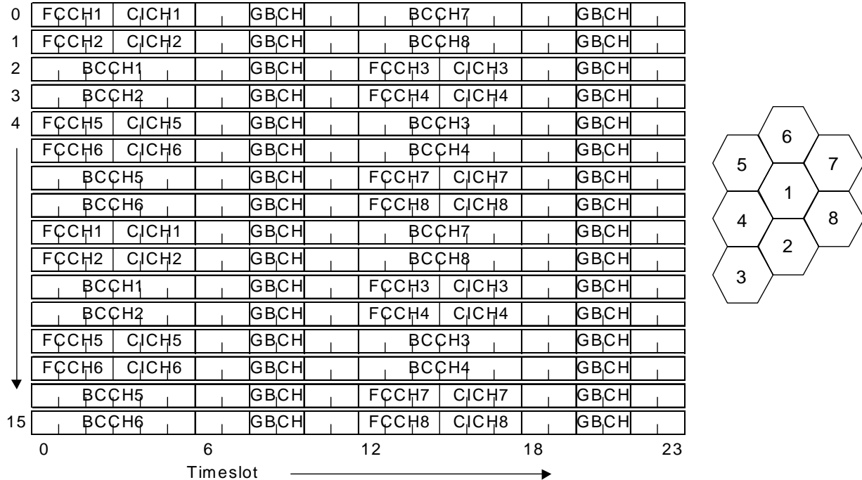
Figure 7.1: Scheduled FCCH and BCCH measurements for neighbouring spot beams
