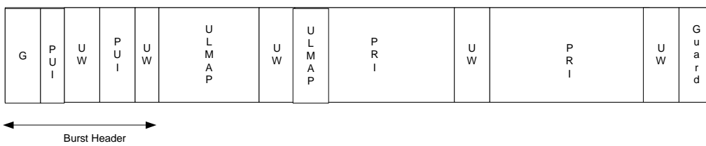
(e) PNB3(5,12) Downlink with UL-MAP
