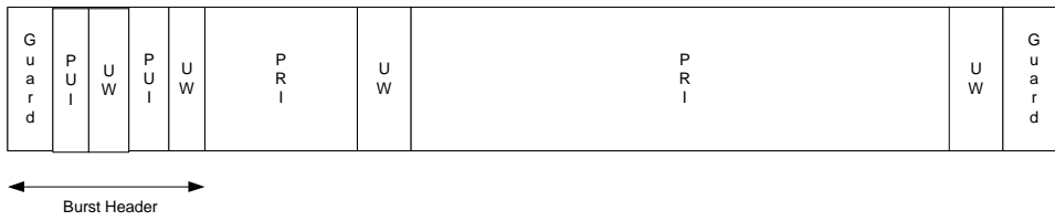
(a) PNB3(5,3) Downlink
