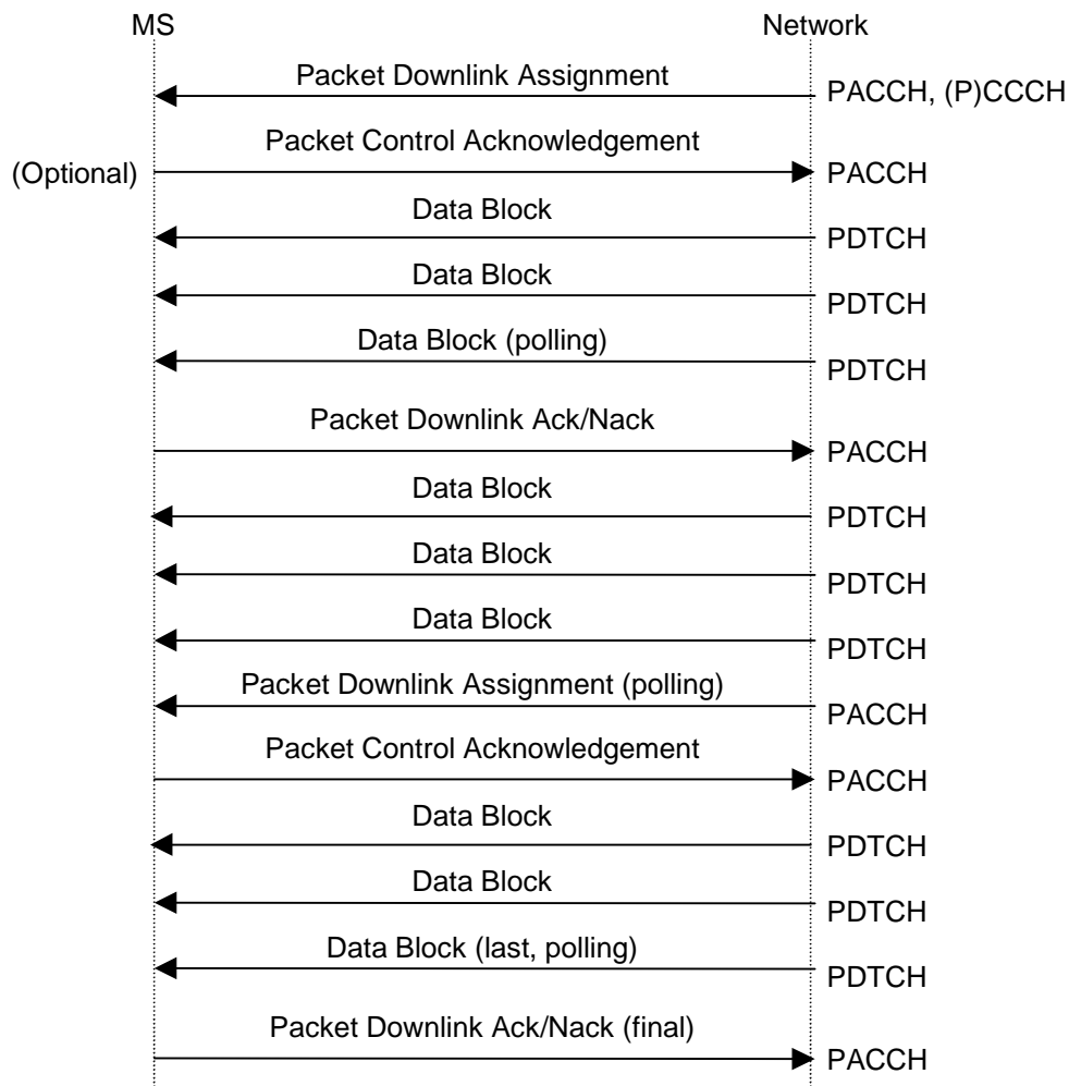
Figure 13: An example of downlink data transfer
