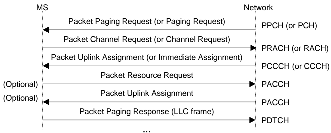
Figure 12: Paging message sequence for Paging, downlink packet transfer
