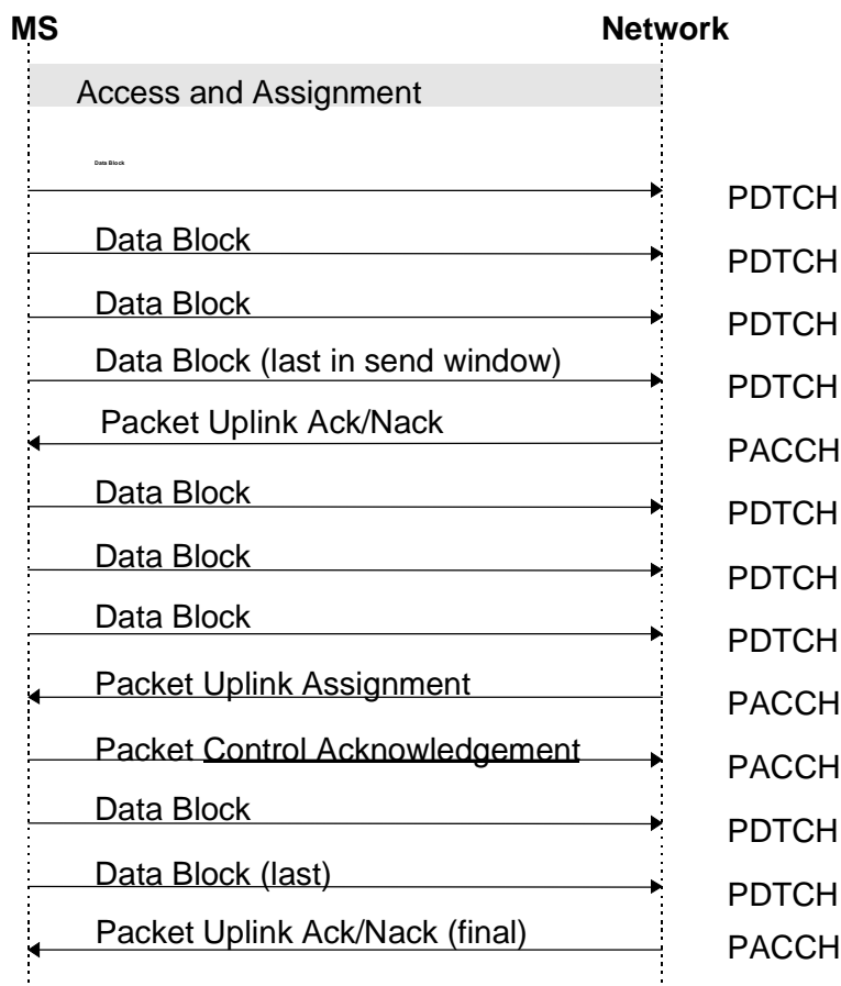
Figure 11: An example of dynamic allocation uplink data transfer
