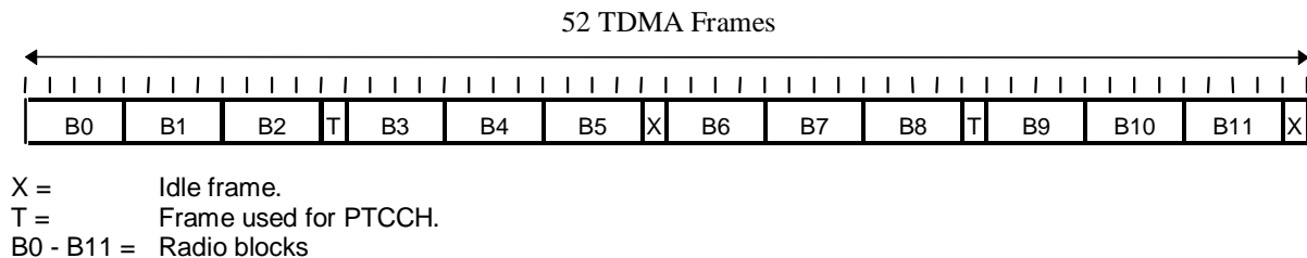
Figure 2: Multiframe structure for PDCH
