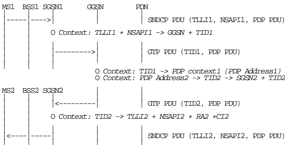
Figure B.3: MS-to-MS Data Routing via the Same GGSN
