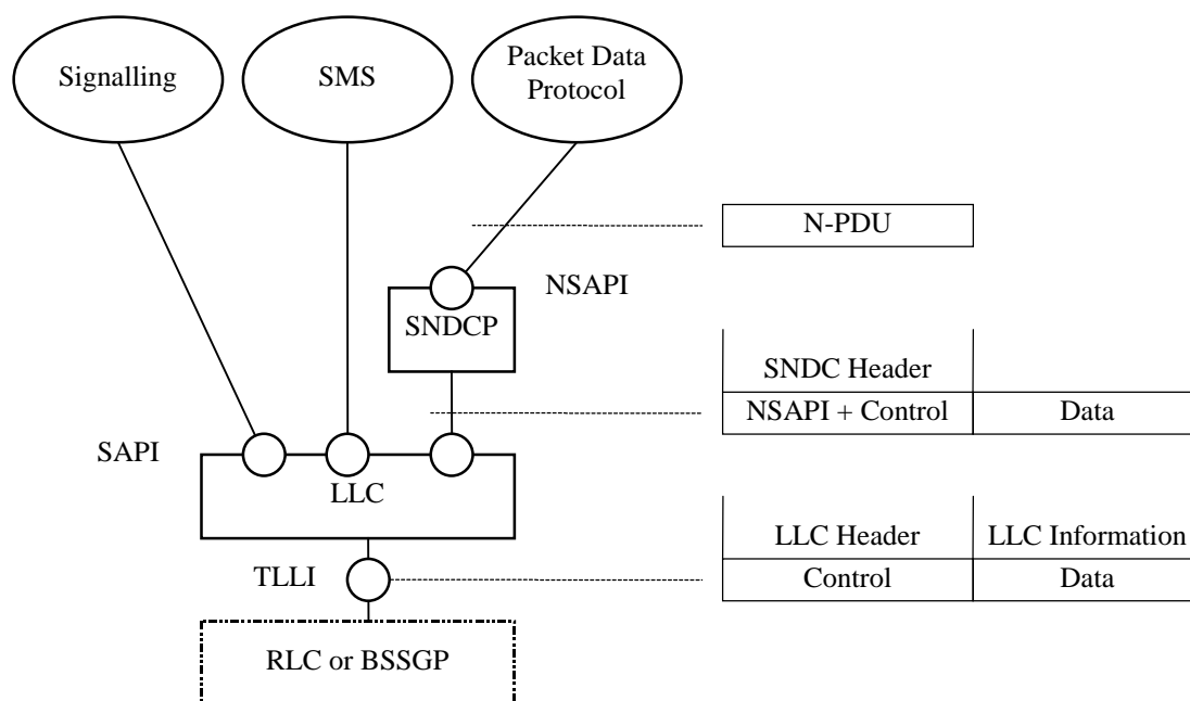
Figure 46: Multiplexing of Network Protocols
