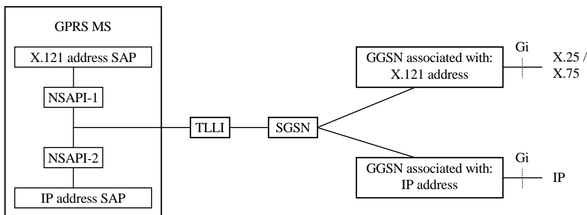
Figure 51: Use of NSAPI and TLLI
