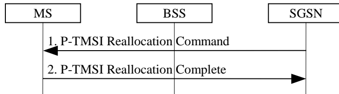
Figure 24: P-TMSI Reallocation Procedure
