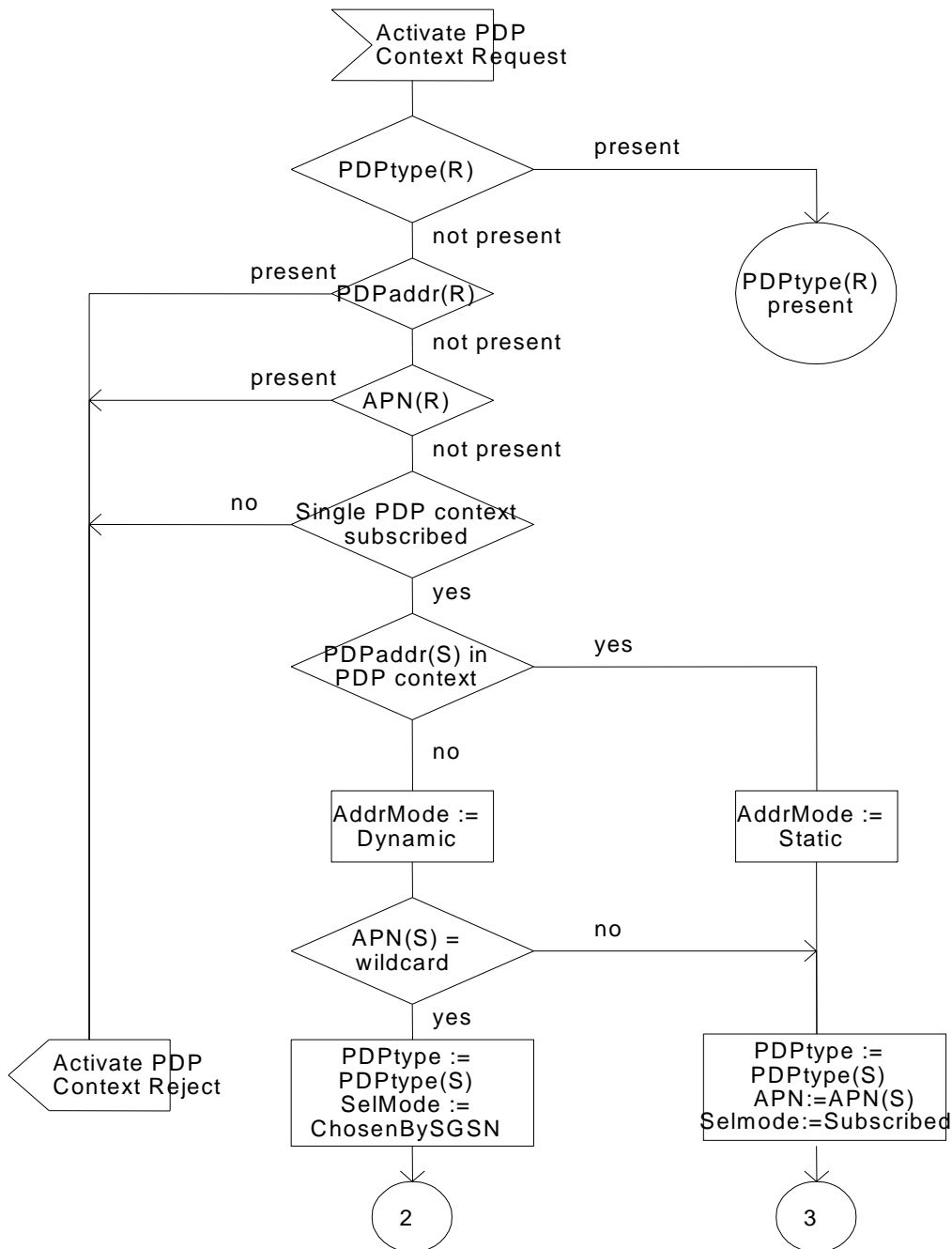
Figure A.1: SDL Diagram 1
