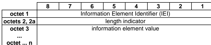
Figure 8/GSM 08.16: Information element structure, TLV format
