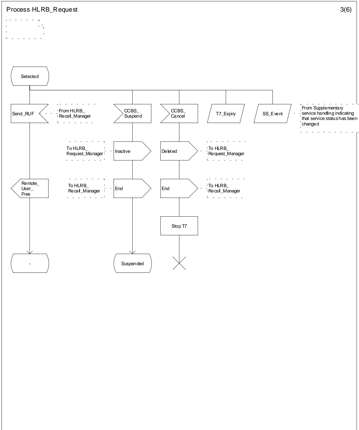
Figure 11.2.2.3: Process HLRB_REQUEST (sheet 3 of 6)
