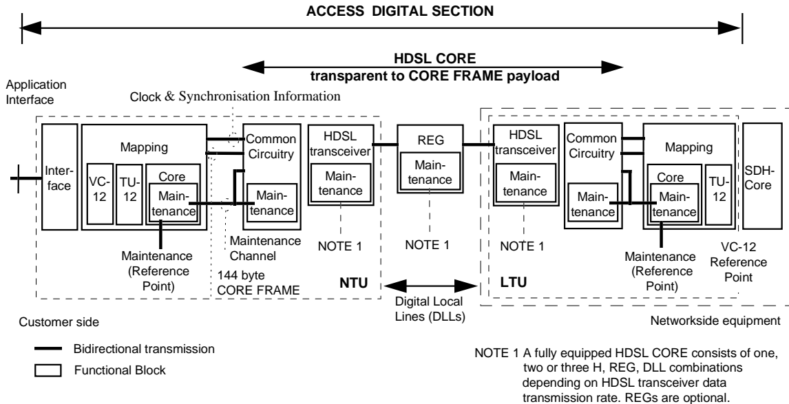
Figure 47: Access Section for TU-12 transport employing HDSL technology
