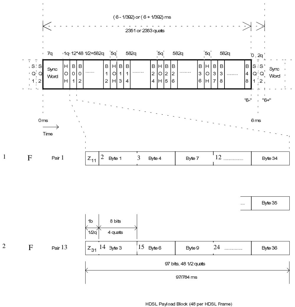
Figure C.1: Frame structure of the two pair system for 784 kbit/s
