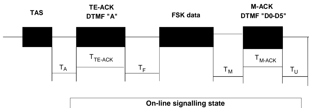
Figure A.1: Timing requirements
