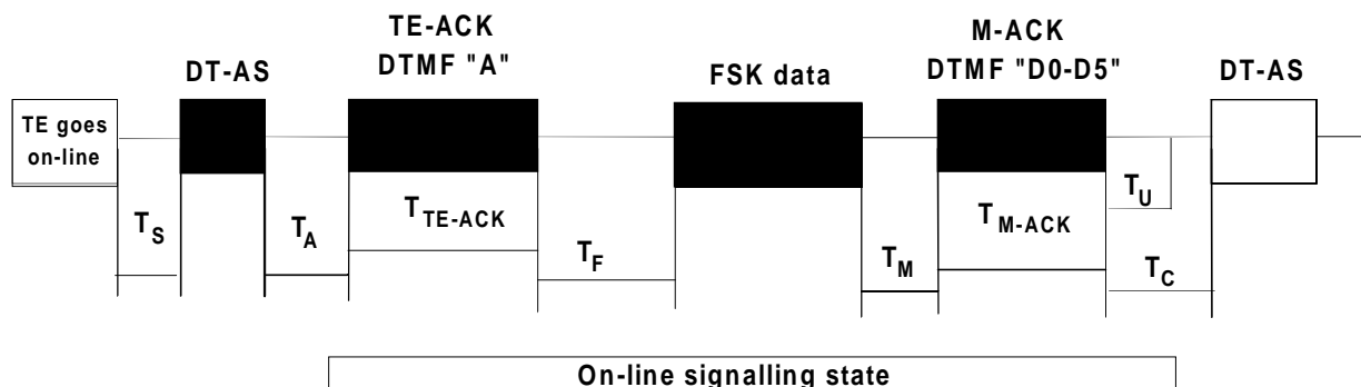
Figure A.2: Timings following reception of Future CPE(TE) ID parameter
