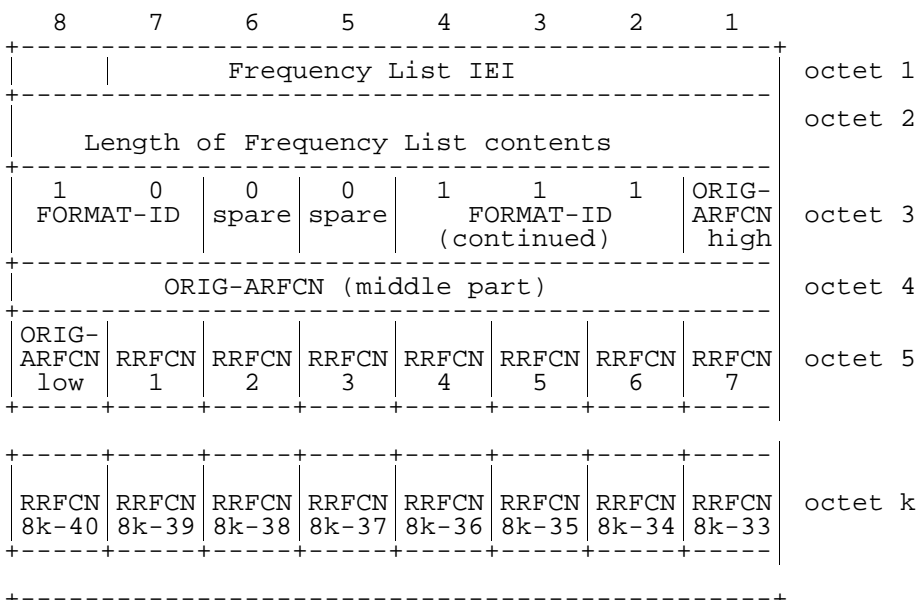
Figure 10.5.40/3GPP TS 04.08: Frequency List information element, variable bit map format
