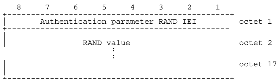
Figure 10.5.75/3GPP TS 04.08: Authentication Parameter RAND information element
