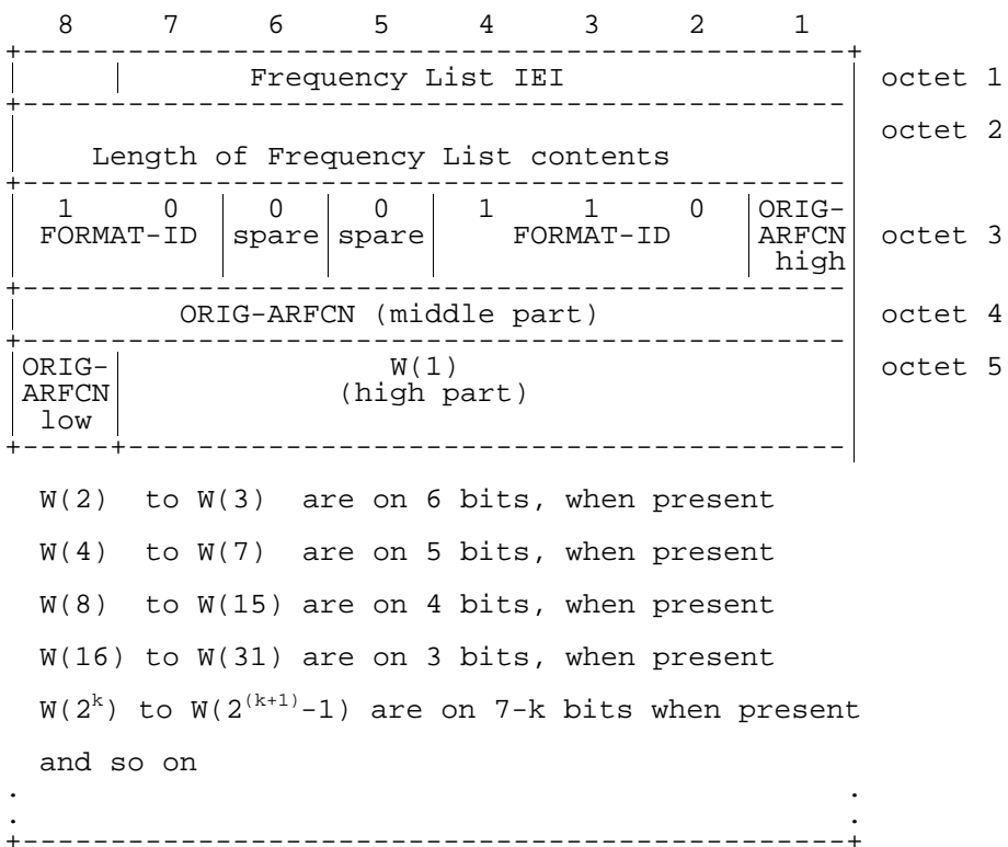
Figure 10.5.39/3GPP TS 04.08: Frequency List information element (Range 128 format)
