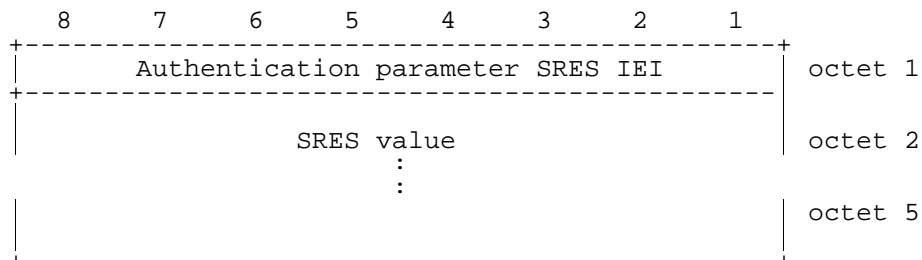
Figure 10.5.76/3GPP TS 04.08: Authentication Parameter SRES information element
