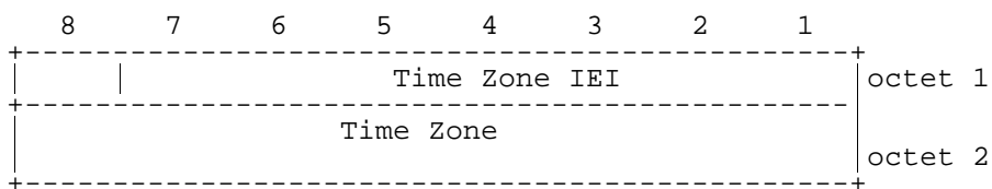
Figure 10.5.83/3GPP TS 04.08: Time Zone information element
