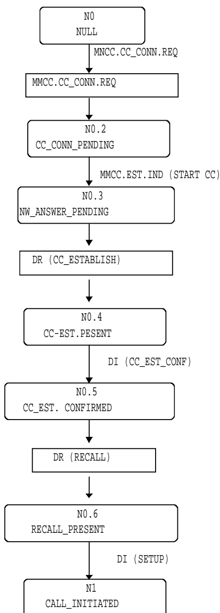
Figure 5.1b.1/3GPP TS 04.08: Overview call control protocol/Network side, extension:
