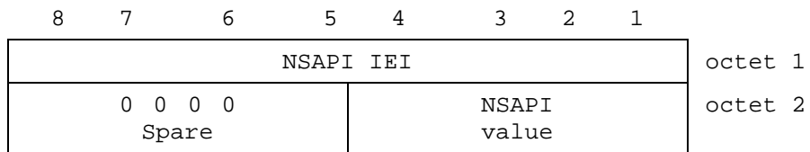
Figure 10.5.135/3GPP TS 04.08: Network service access point identifier information element
