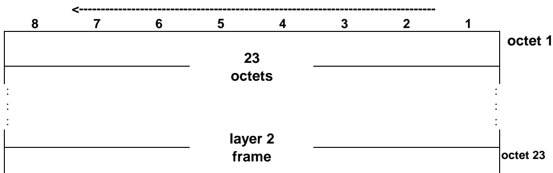
Figure 7.4: FACCH/SDCCH uplink block format
