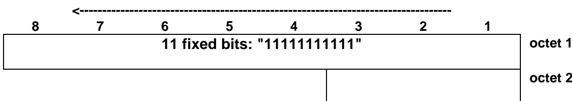
Figure 7.11 (sheet 2 of 2): PTCCH uplink block format
