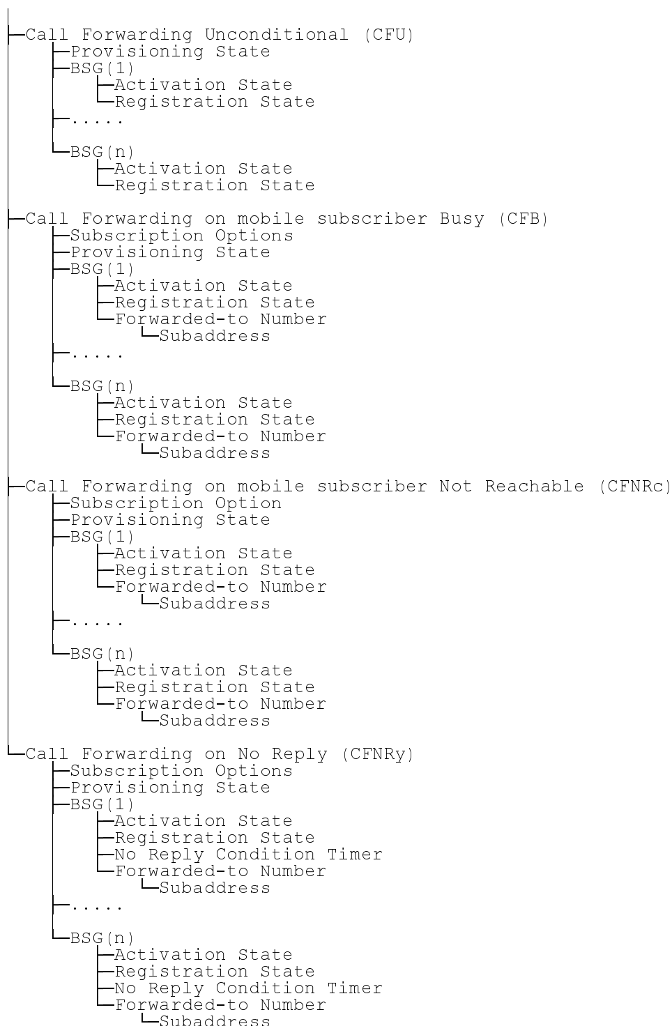
Figure 3: Forwarding Info
