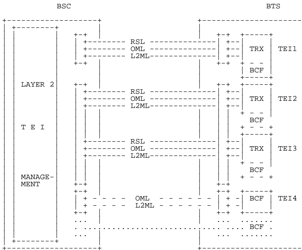
Figure 6.2/08.52: Logical L2 links of A-bis interface
